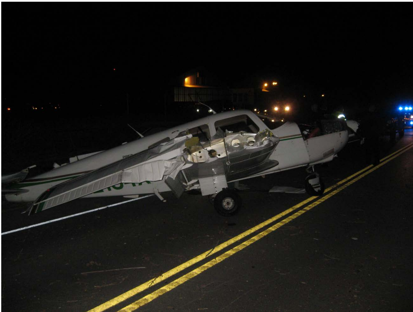
Photo 2 – View of right side of airplane showing right wing damage
