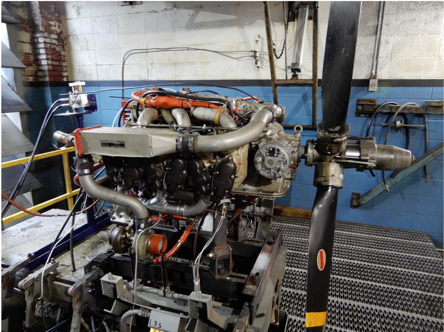
Photo 8 – Engine, Mounted on Test Stand (NTSB Photo)
