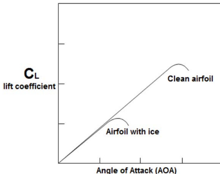
FIGURE 3-5. LIFT CURVE
