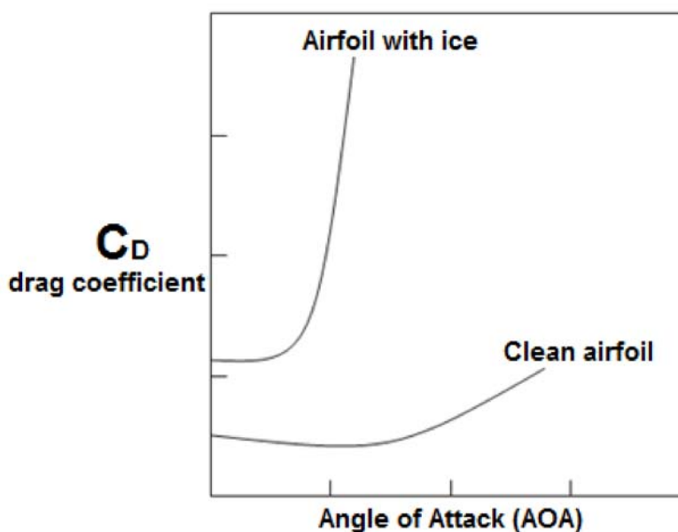
FIGURE 3-6. DRAG CURVE
