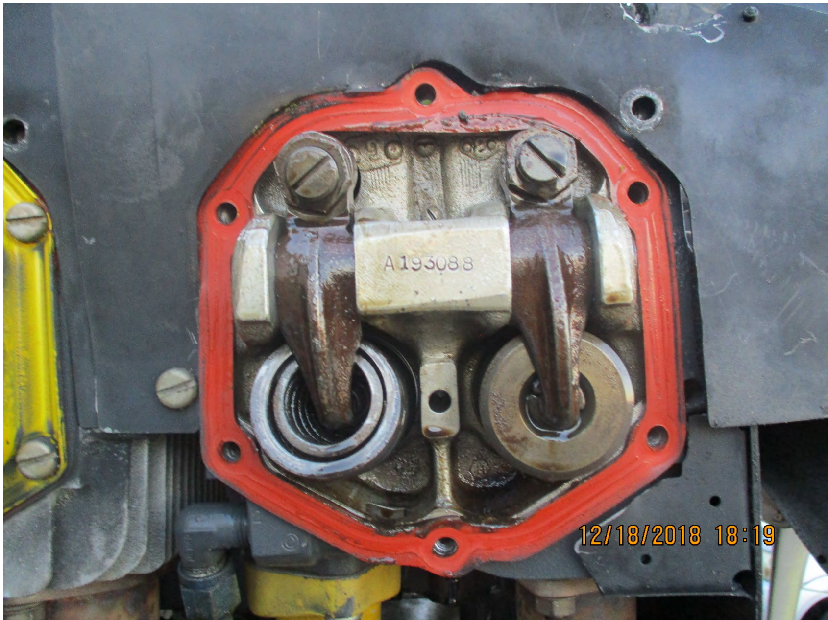
Photo 4 – View of No. 1 Cylinder after Rocker Cover Removed (Photo Courtesy of FAA)
