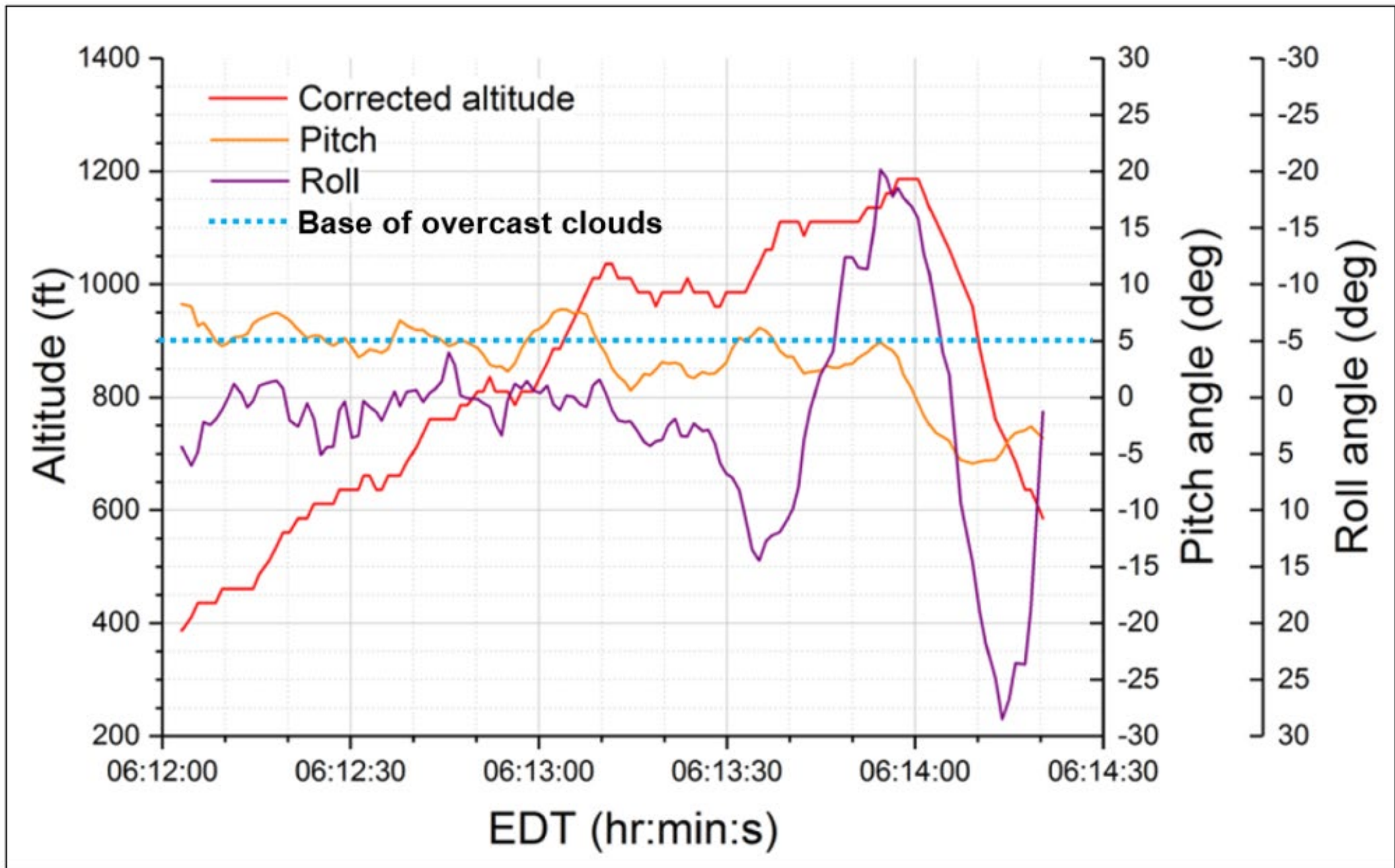
Figure 3: Accident flight altitude, pitch, roll, and cloud layer data (Source: NTSB Performance and Weather Studies)
