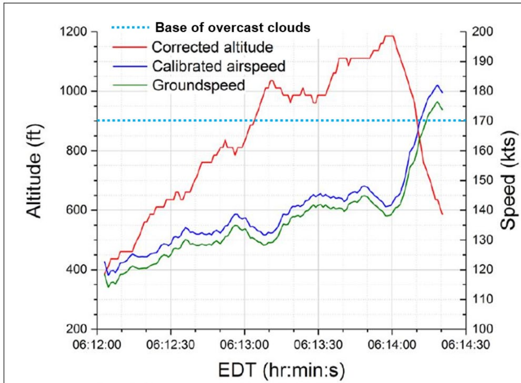
Figure 2: Accident flight altitude, calculated groundspeed and airspeed, and cloud layer data (Source: NTSB Performance and Weather Studies)
