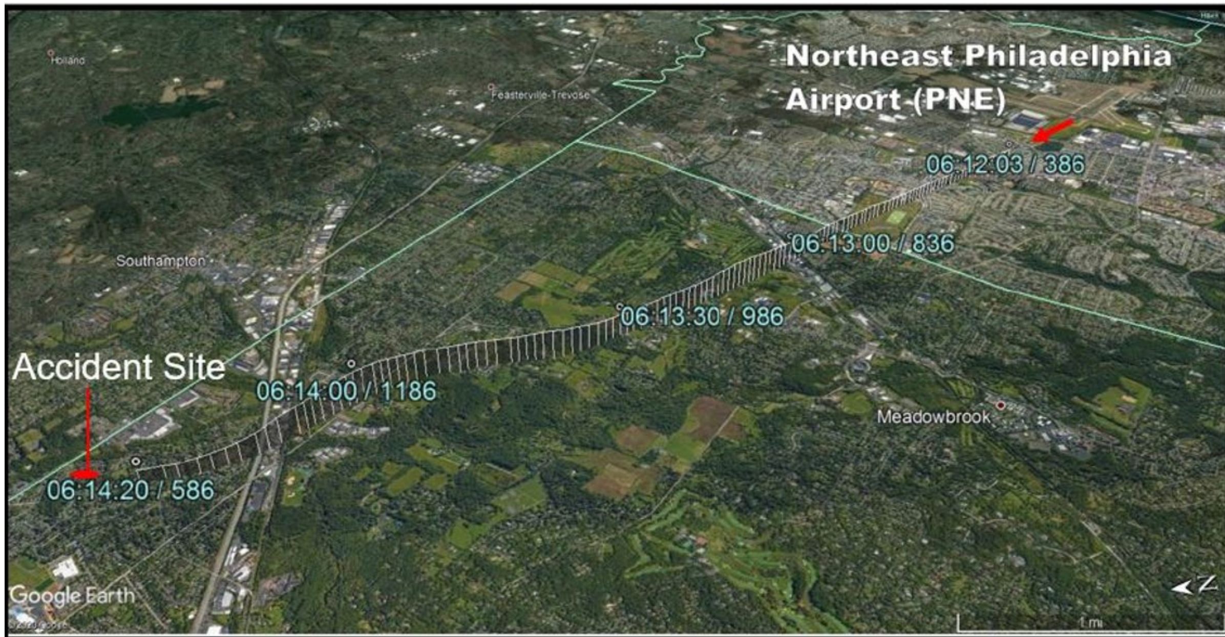
Figure 1: The airplane's flightpath, denoted by the white line with the time and corresponding airplane altitude (ft msl)
