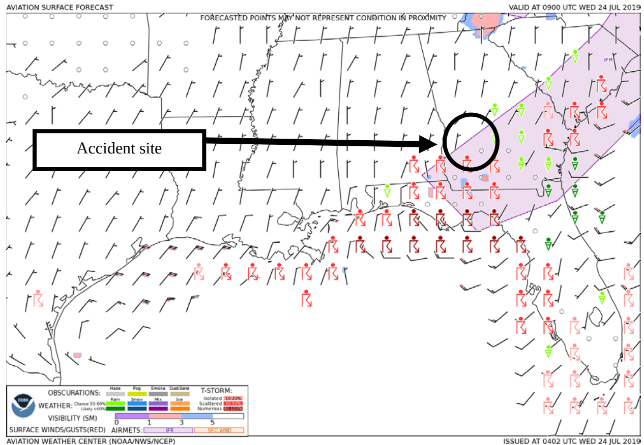
Figure 1 – GFA Surface Forecast valid at 0500 EDT with forecast issued at 0002 EDT
