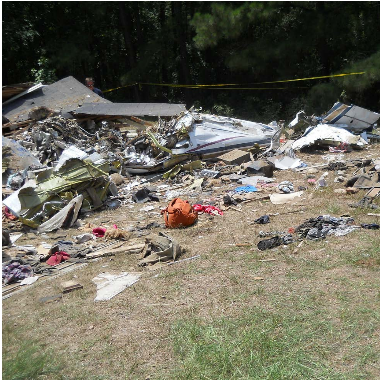
Photo 1 – Main Wreckage
