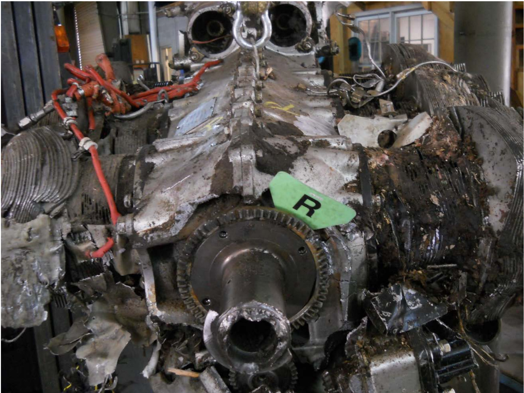
Photo 4 – Right Engine
