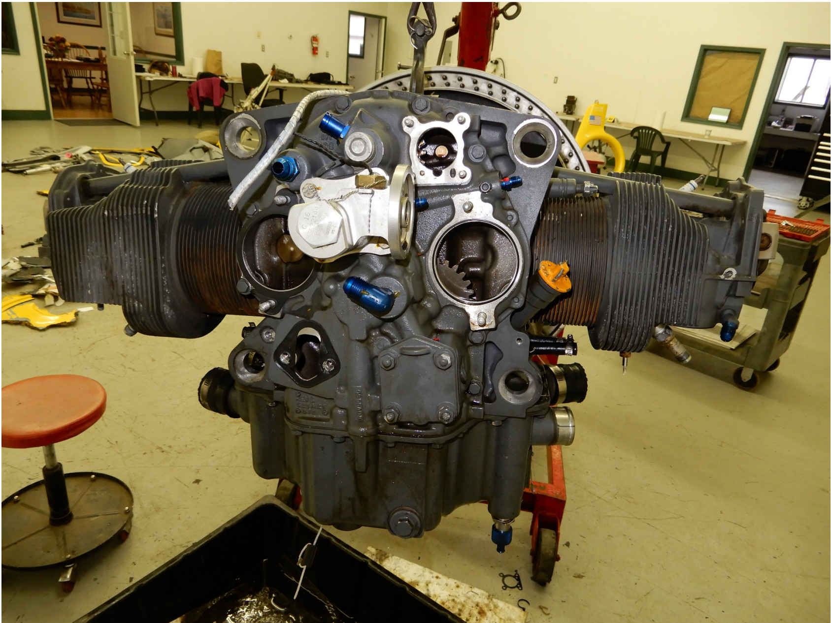
Photo 6 – View of accessory section of engine.
