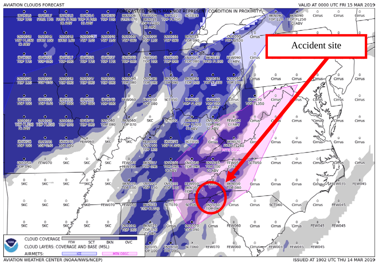
Figure 4 – GFA Aviation Clouds Forecast valid at 2000 EDT with forecast issued at 1502 EDT
