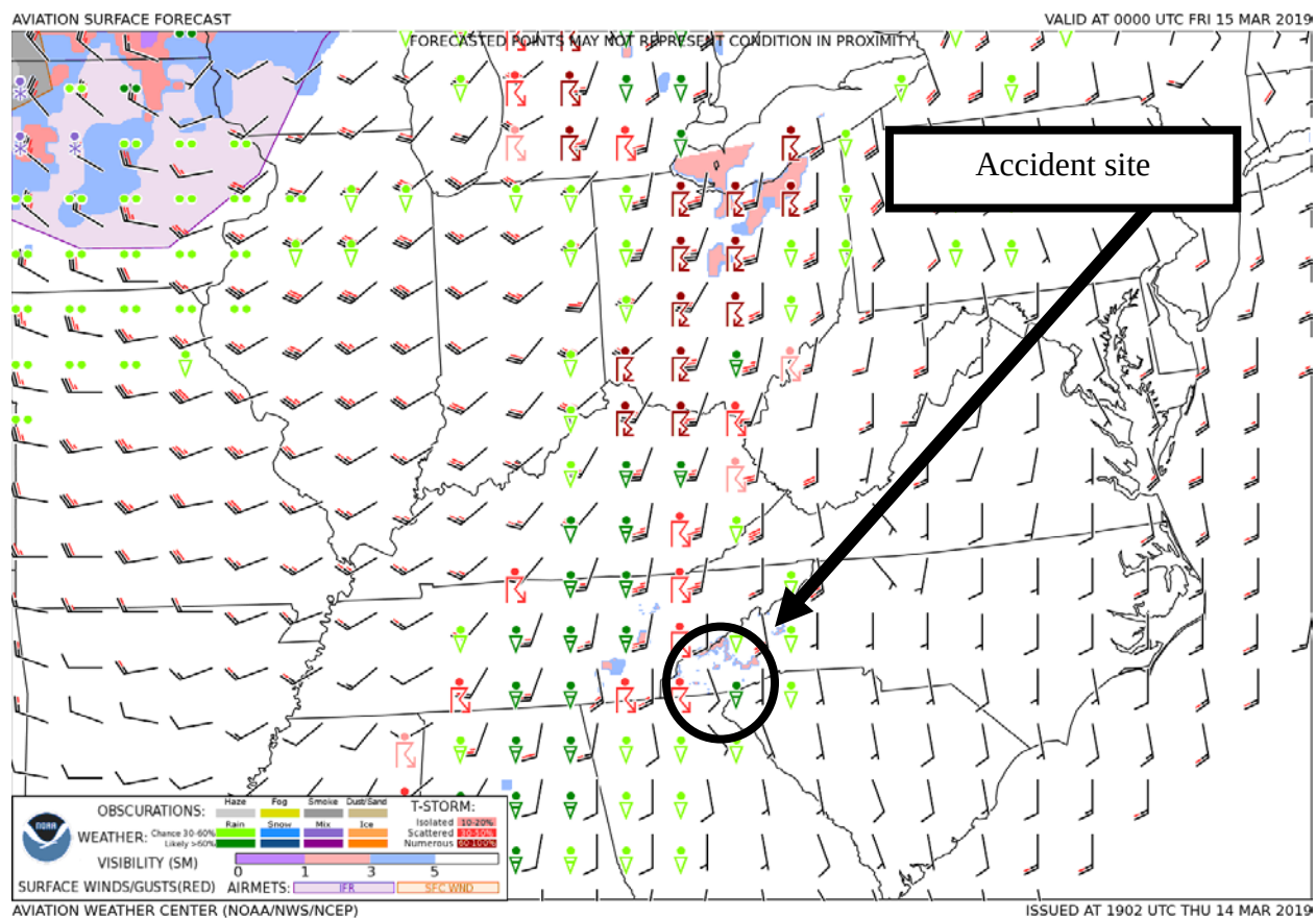
Figure 2 – GFA Surface Forecast valid at 2000 EDT with forecast issued at 1502 EDT
