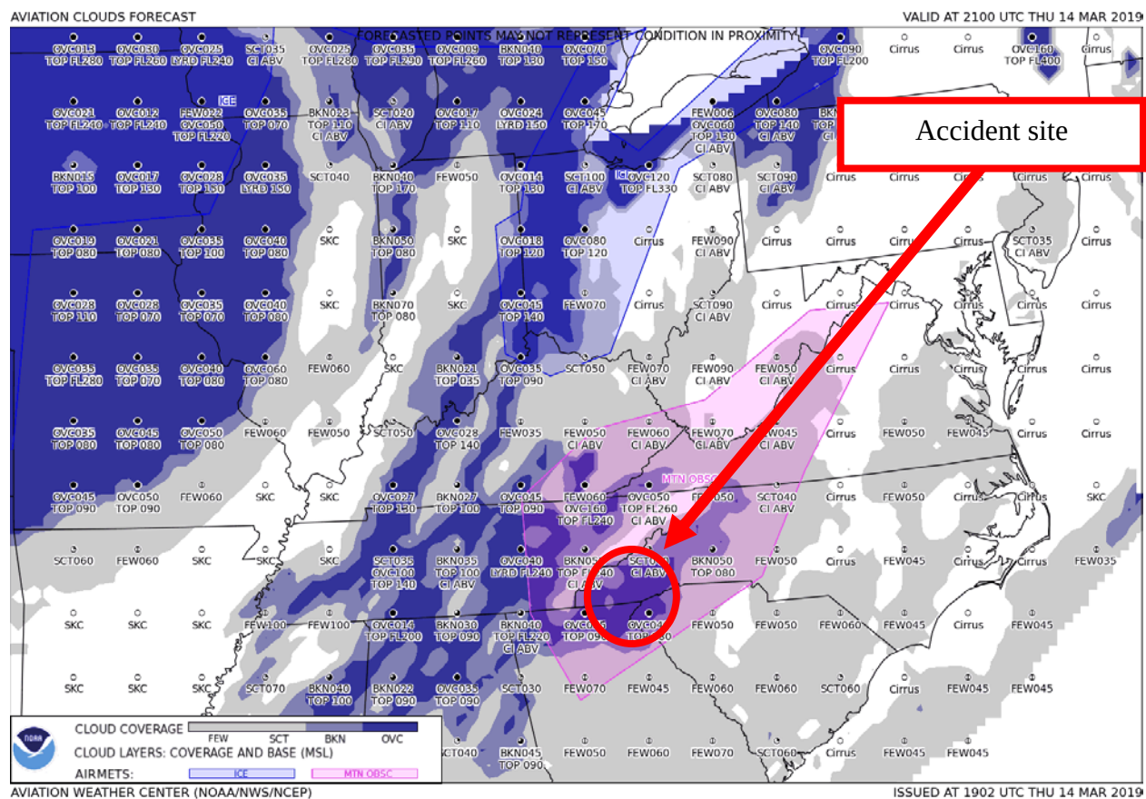
Figure 3 – GFA Aviation Clouds Forecast valid at 1700 EDT with forecast issued at 1502 EDT
