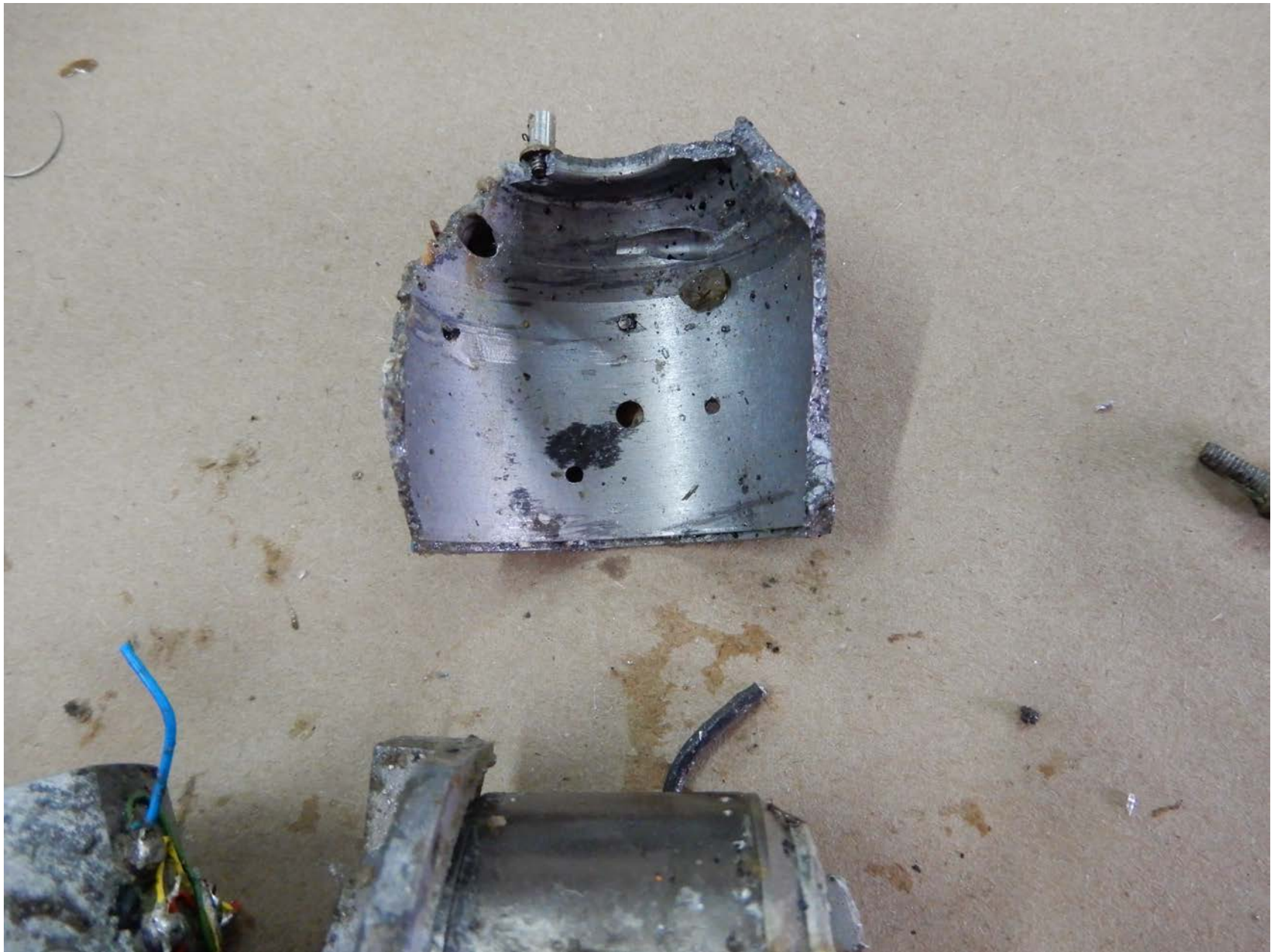
Photo 6 – View of gyroscopic scoring from primary attitude indicator housing
