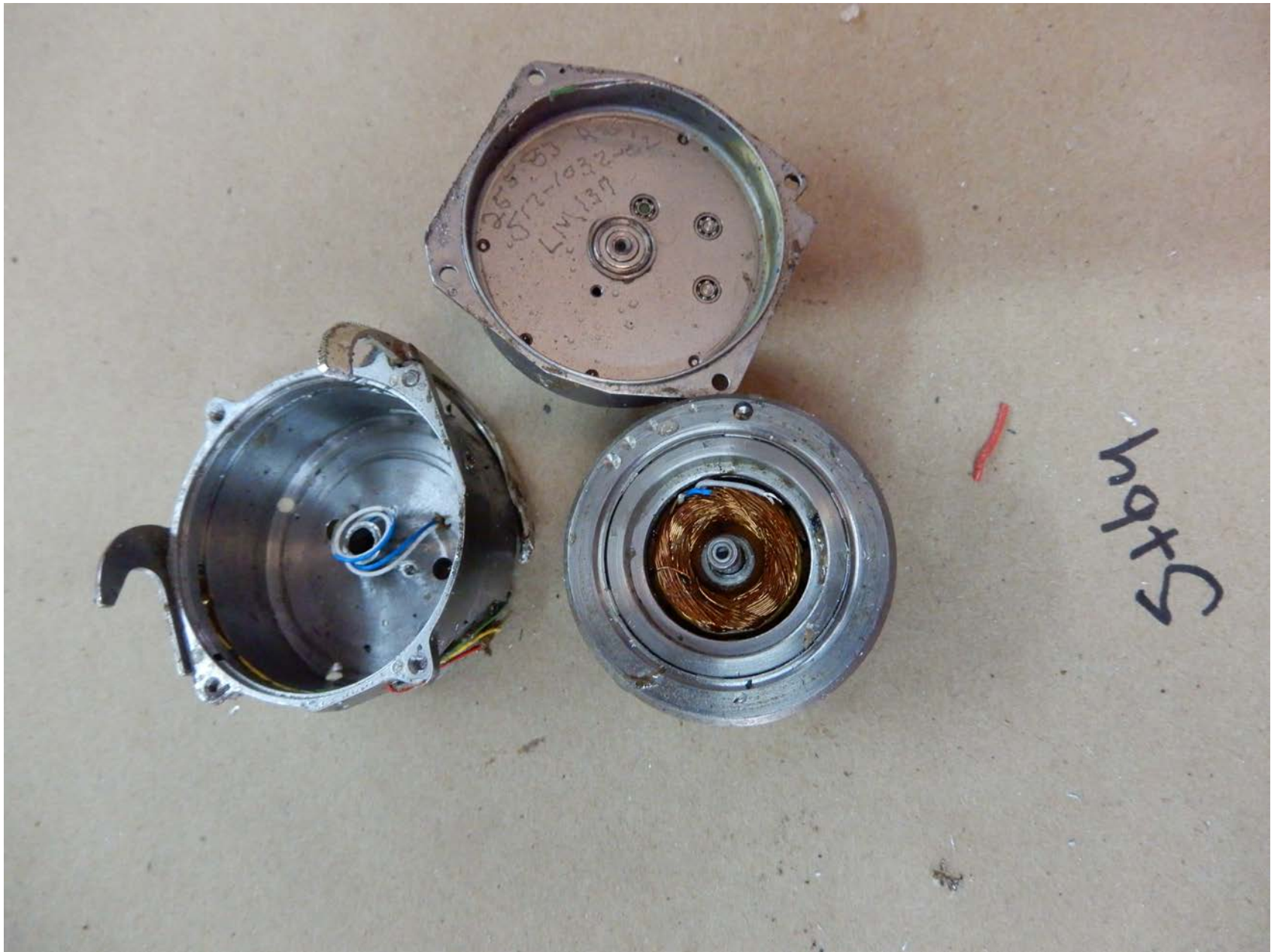
Photo 5 – View of Gyroscopic Scoring from Standby Attitude Indicator
