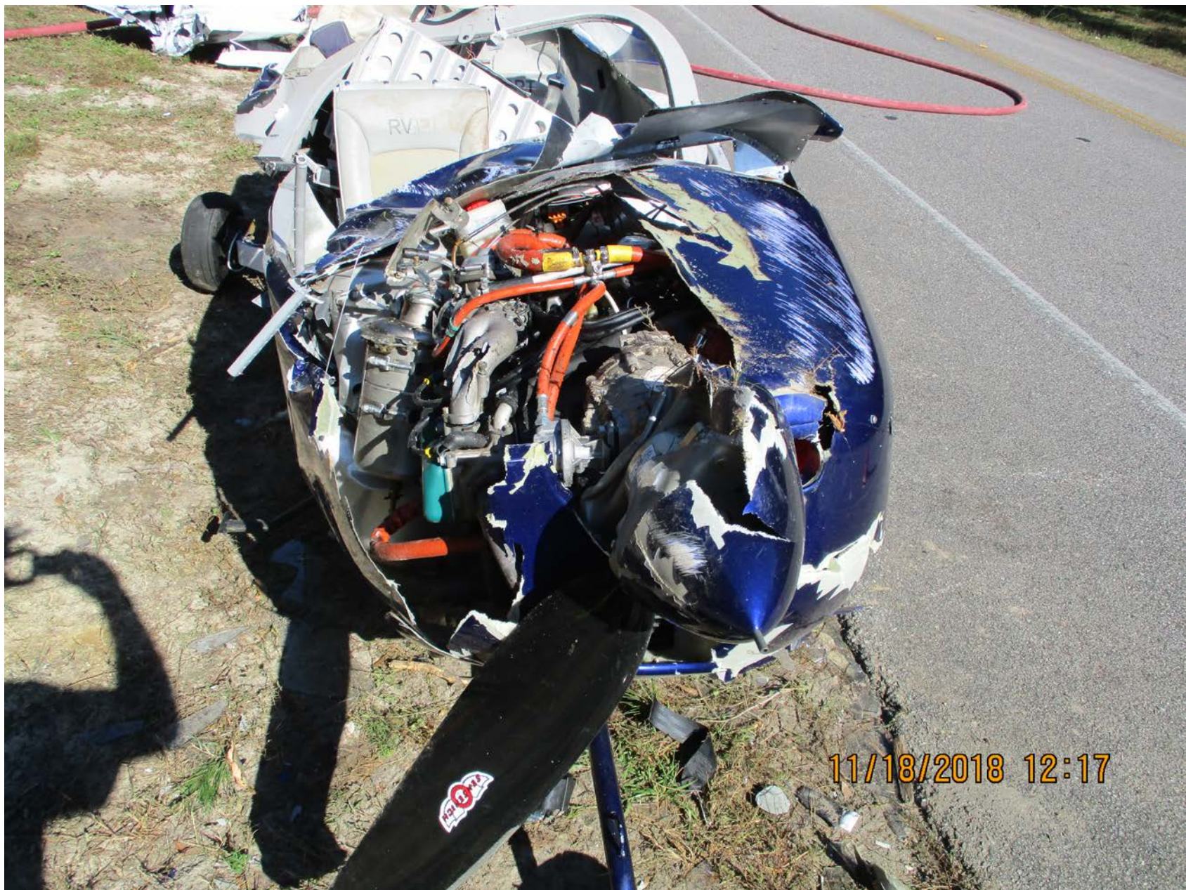
Photo 5 – Engine-Front view
