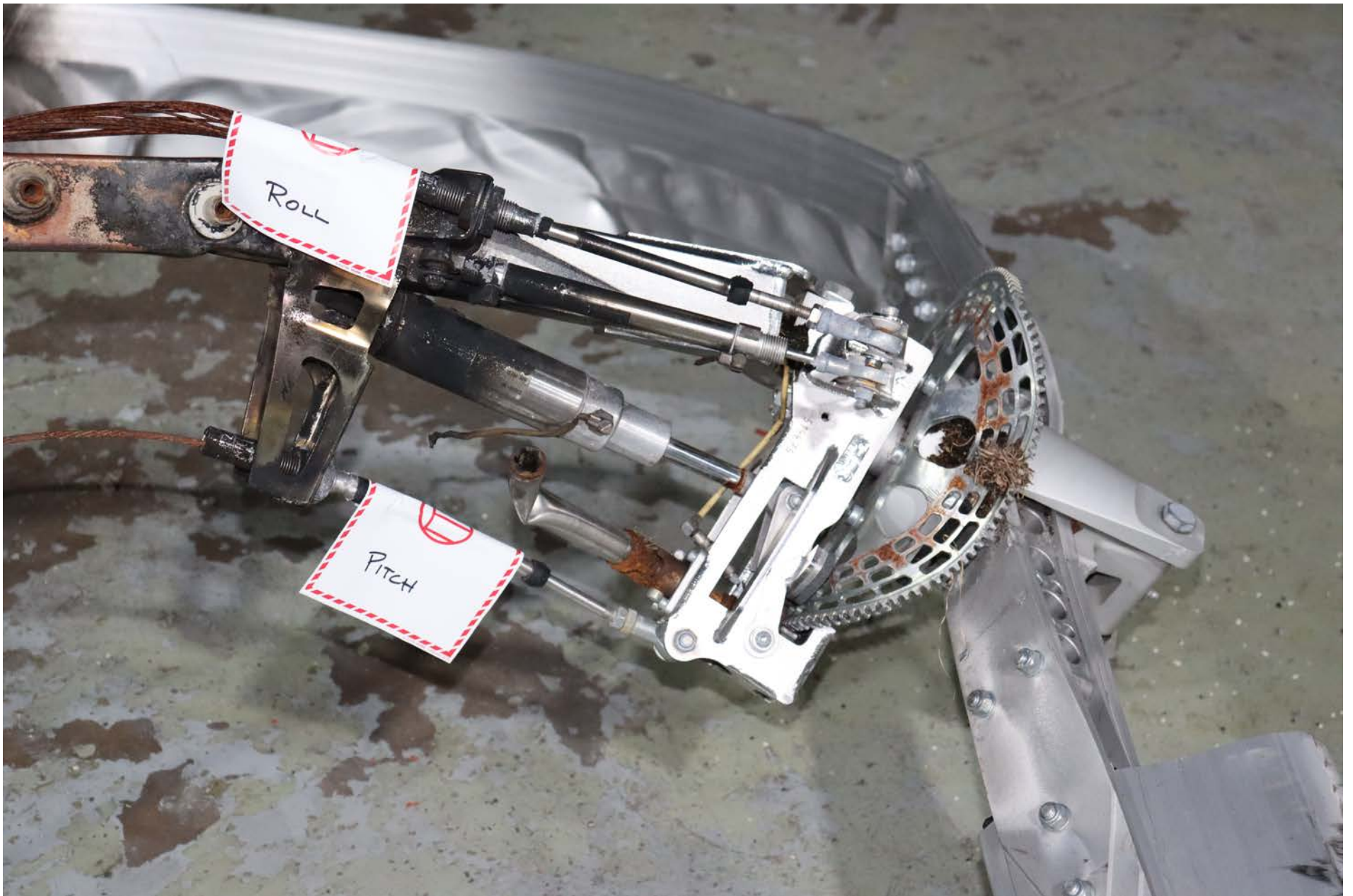
Photo 5 – View of Upper Flight Controls (AutoGyro USA)
