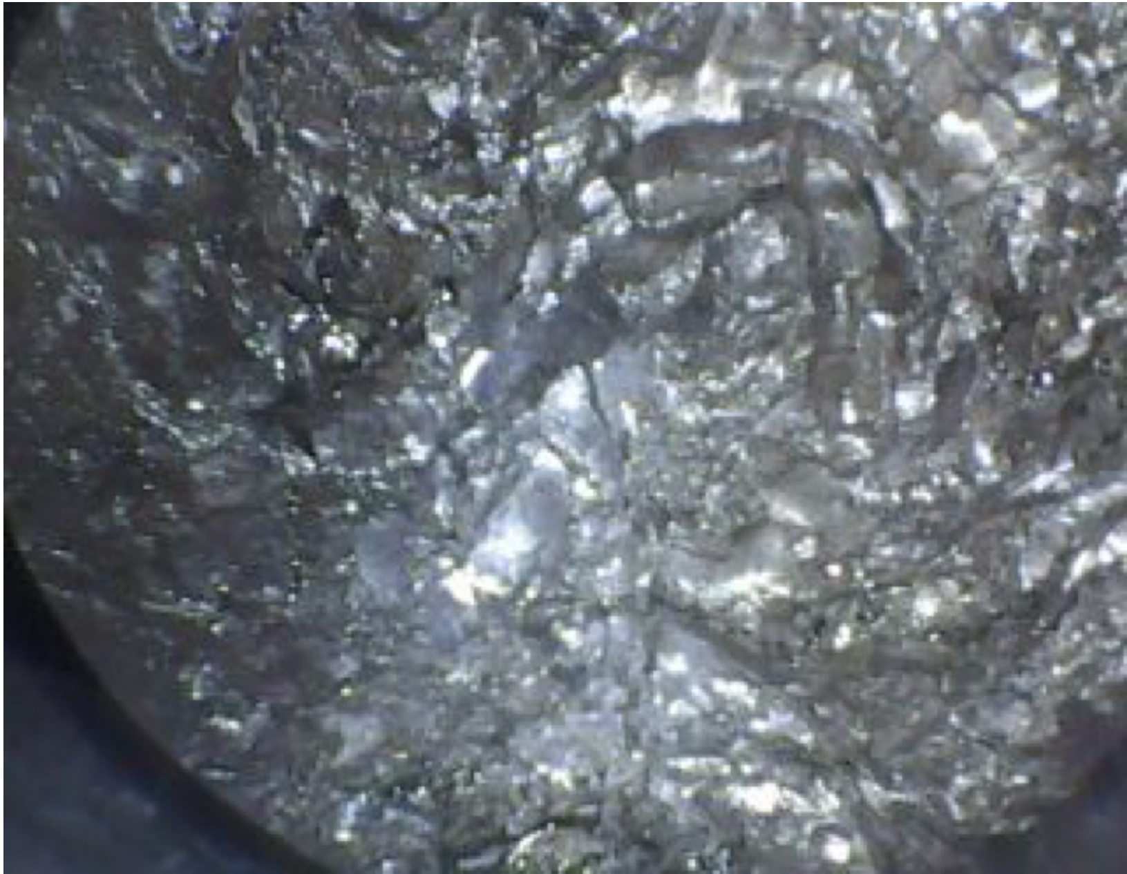
Photo 3 - #4-cylinder, piston.
