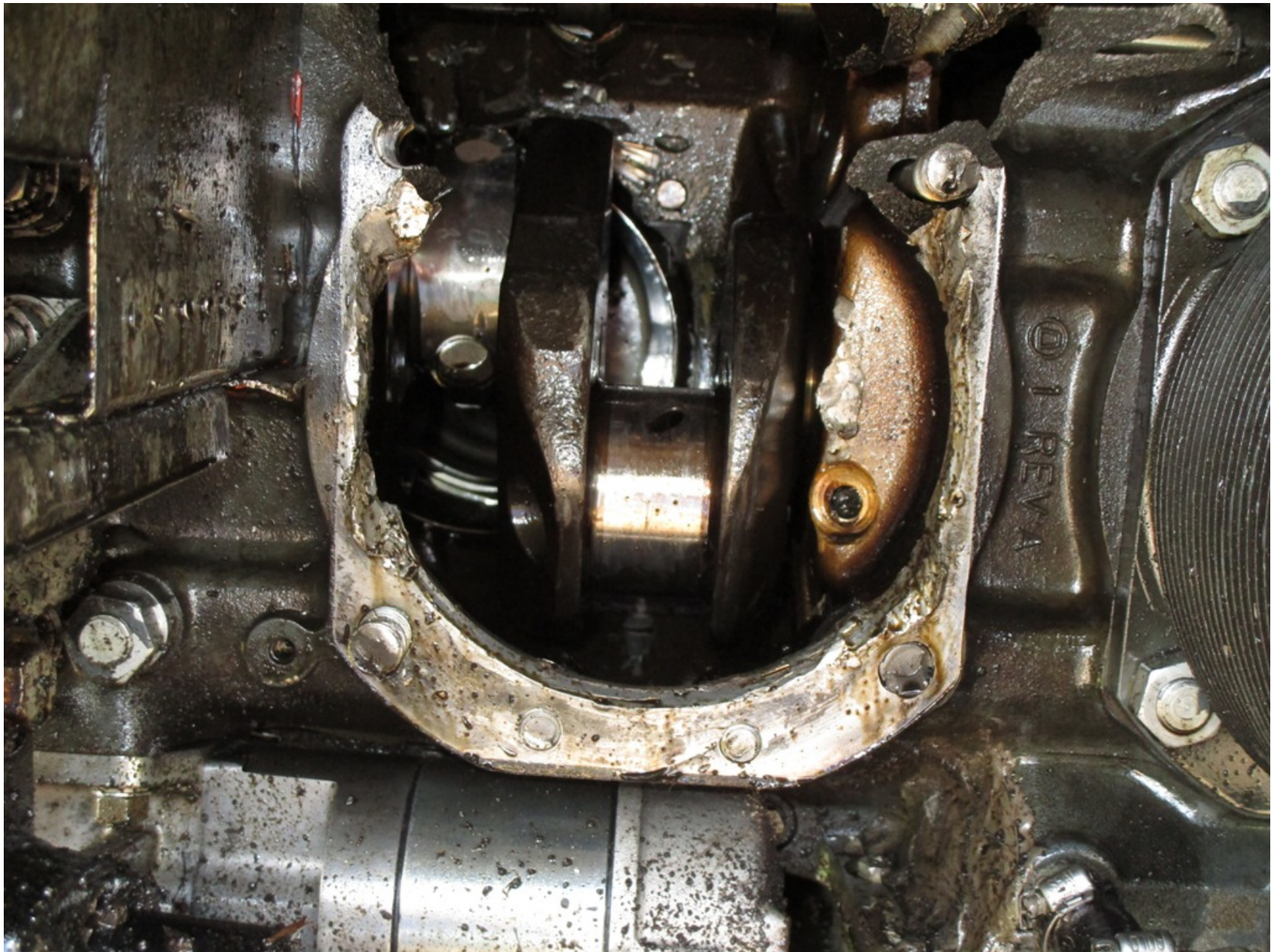
Photo 5 – No. 2 Cylinder Mounting Deck (Photo Credit: FAA)
