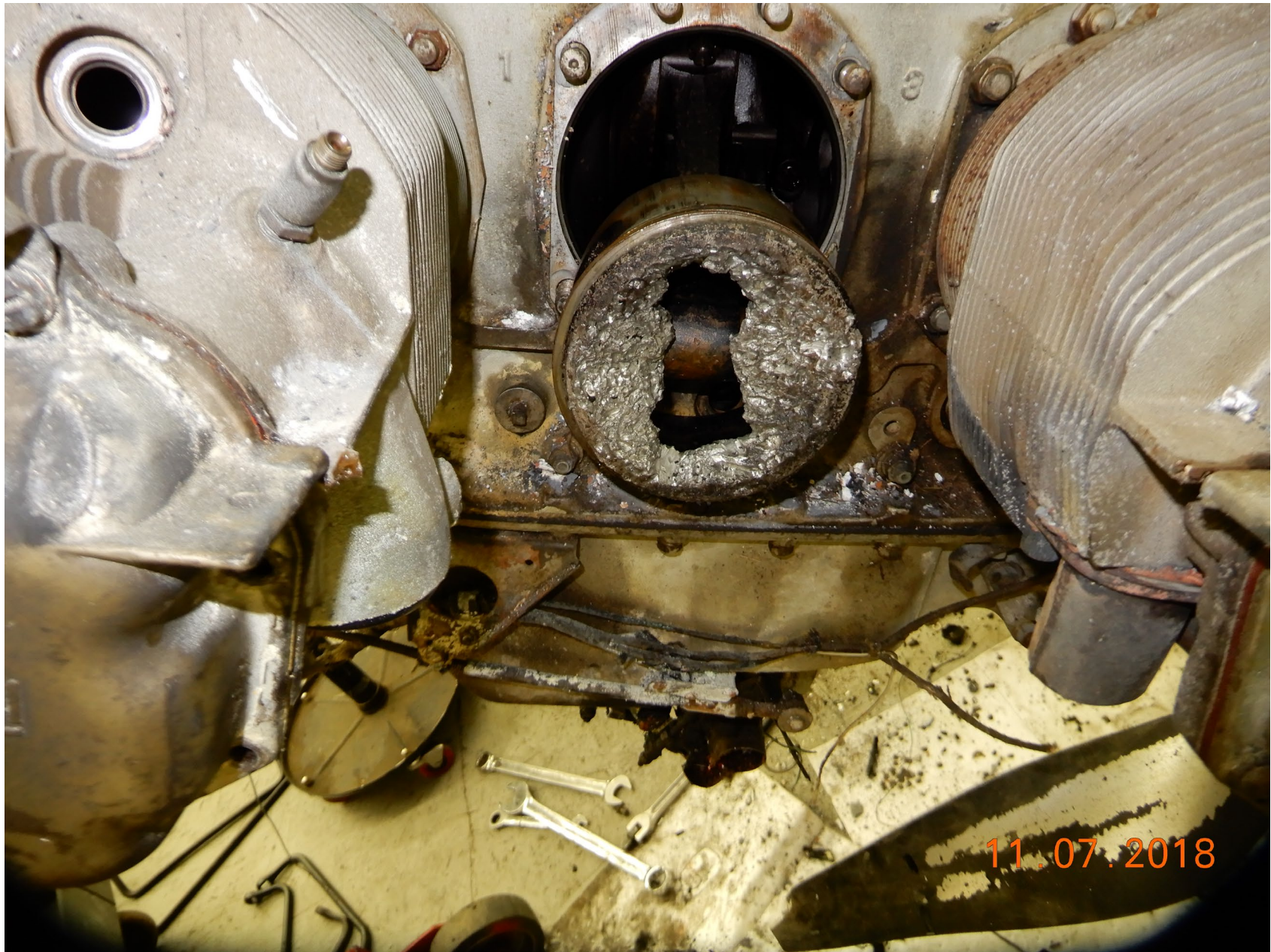
Photo 4 – View of the damage to the No. 3 piston.
