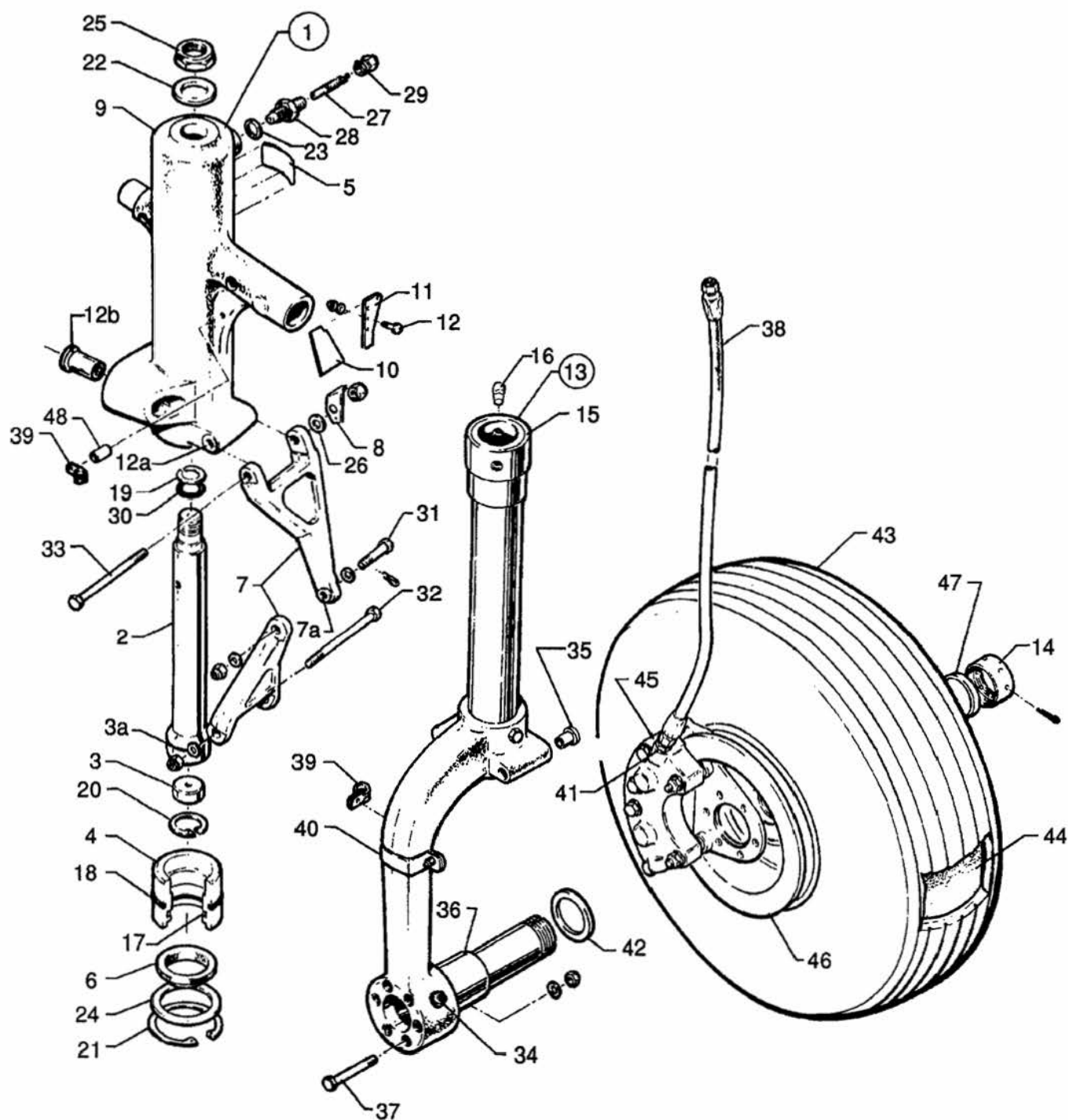
Figure 28. Main Gear Assembly
