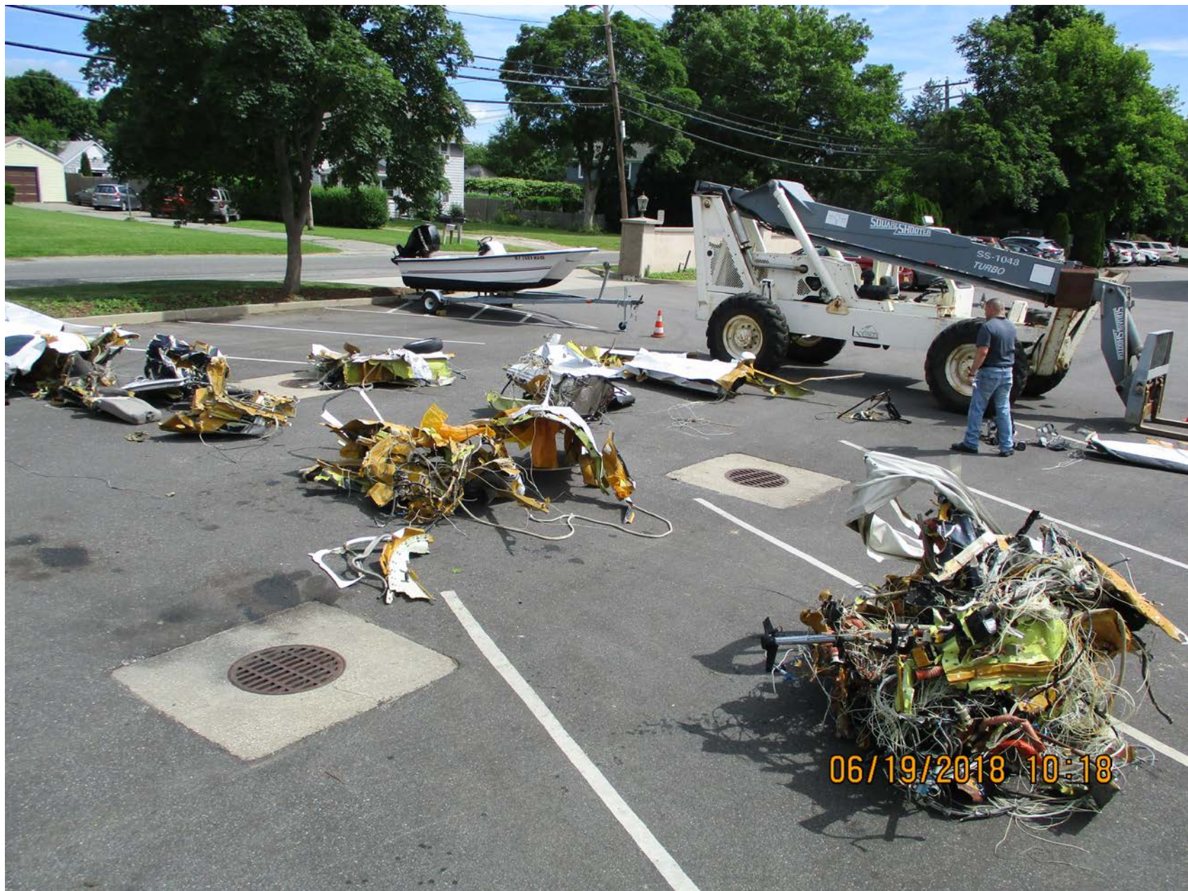
Photo 5 – Airframe parts
