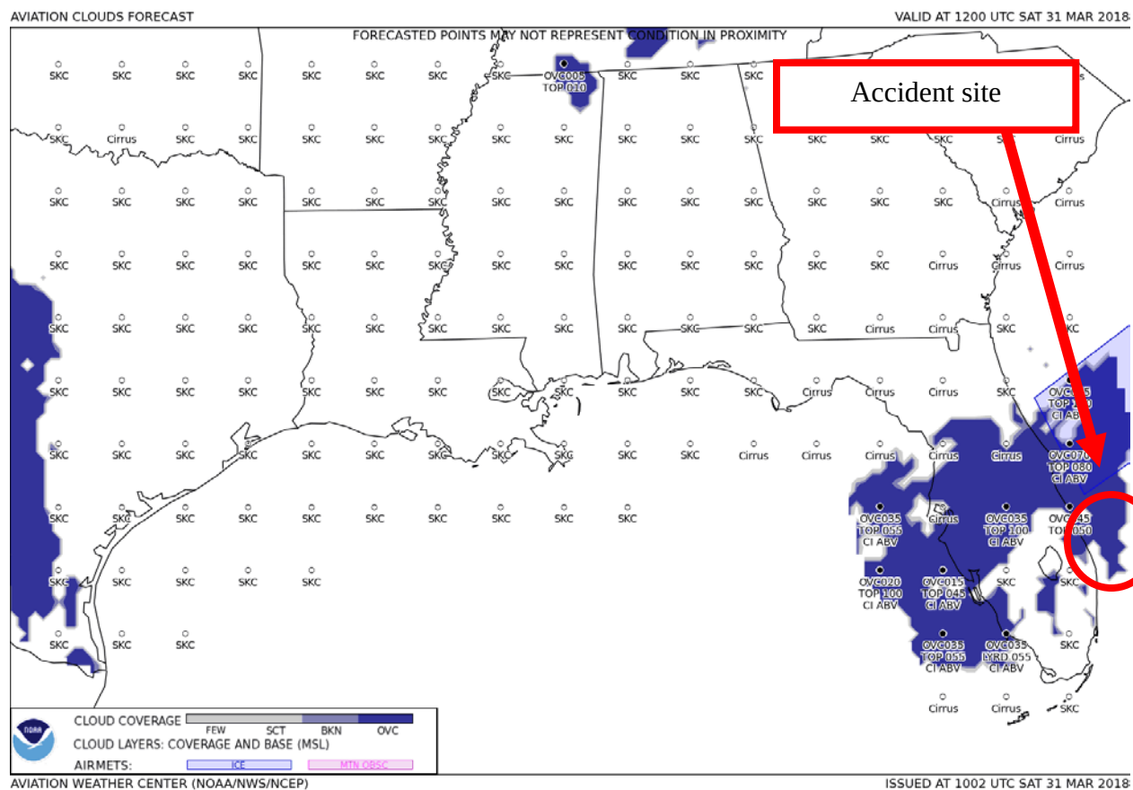
Figure 4 – GFA Aviation Clouds Forecast valid at 0800 EDT with forecast issued at 0602 EDT
