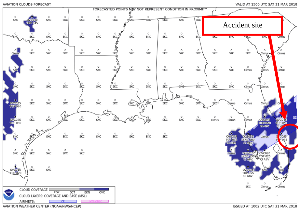
Figure 5 – GFA Aviation Clouds Forecast valid at 1100 EDT with forecast issued at 0602 EDT
