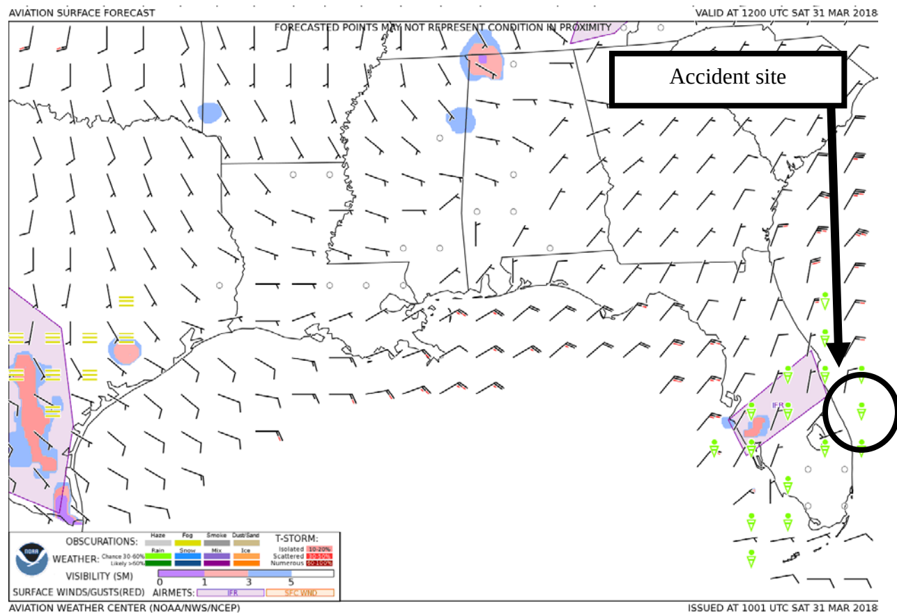
Figure 1 – GFA Surface Forecast valid at 0800 EDT with forecast issued at 0601 EDT
