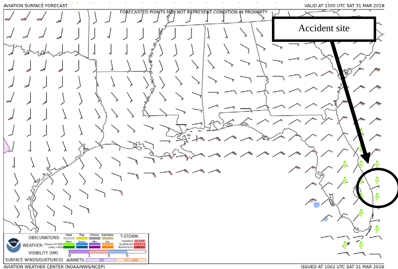
Figure 2 – GFA Surface Forecast valid at 1100 EDT with forecast issued at 0602 EDT
