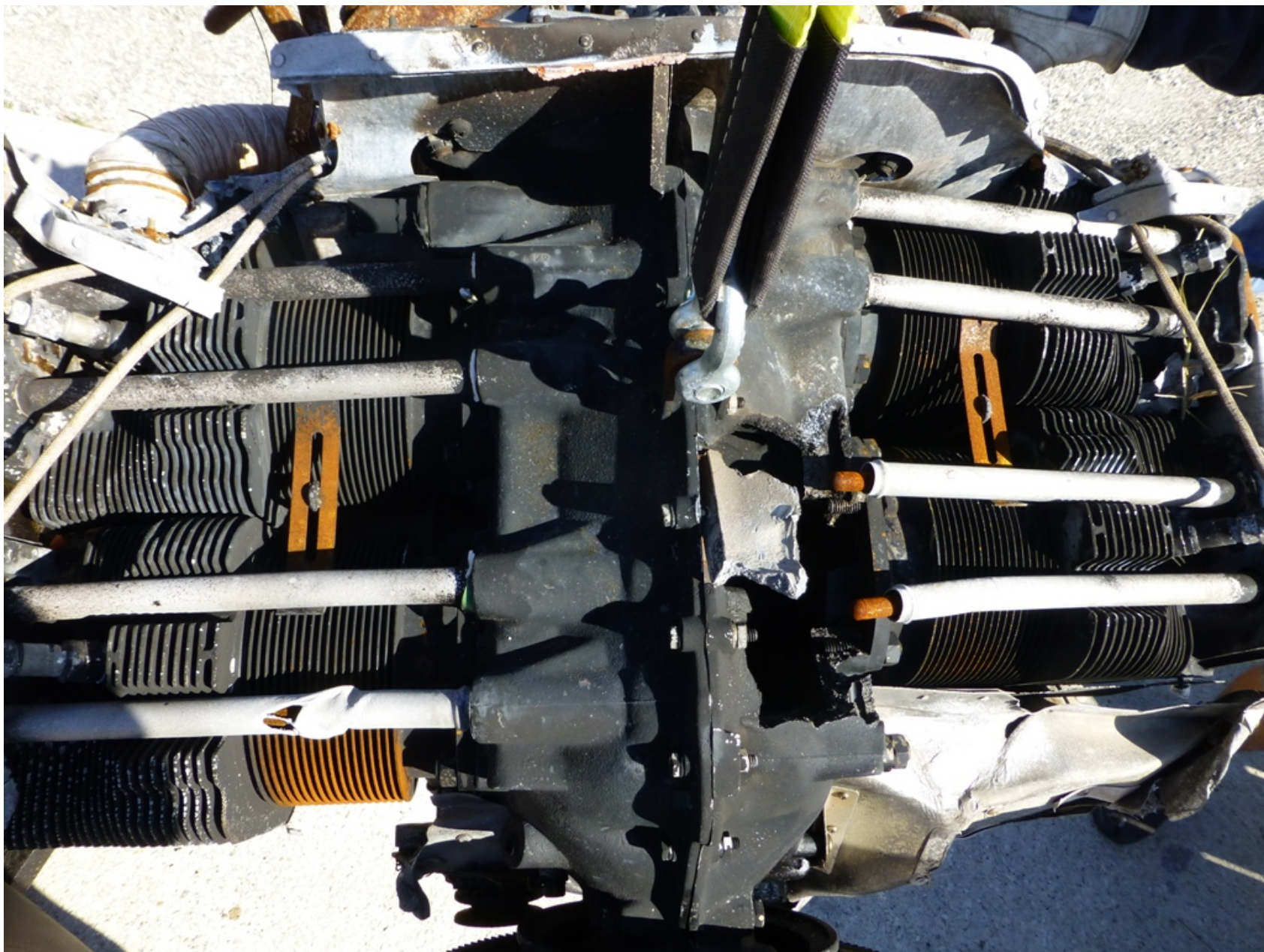
Photo 10 – Engine (NTSB Photo)
