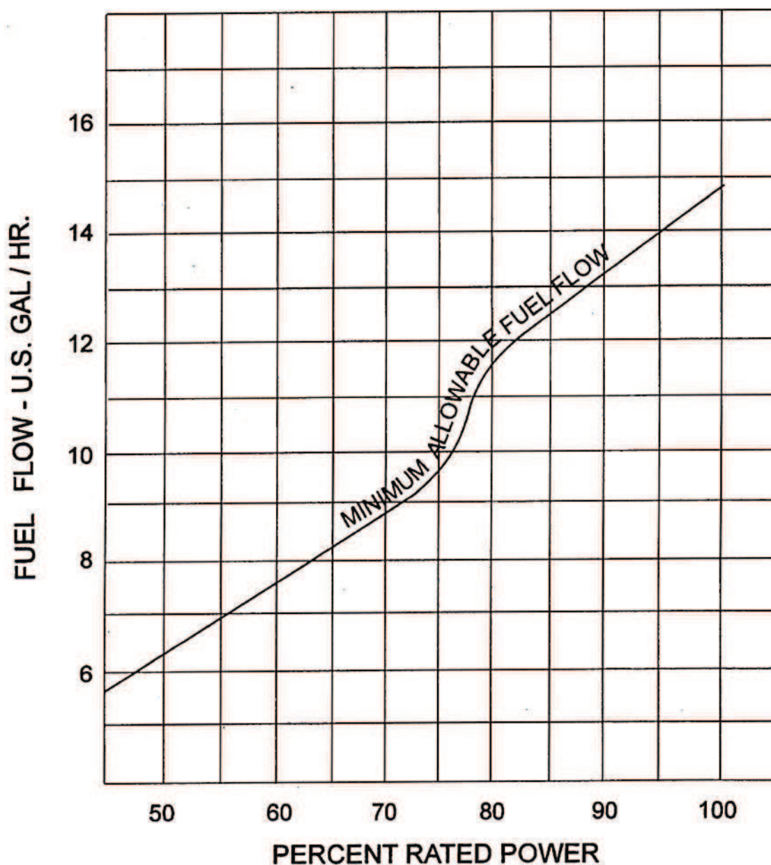
Figure 3-39. Fuel Flow vs Percent Rated Power – O-360-A, -C, -F, -G Series; HO-360-C1A
