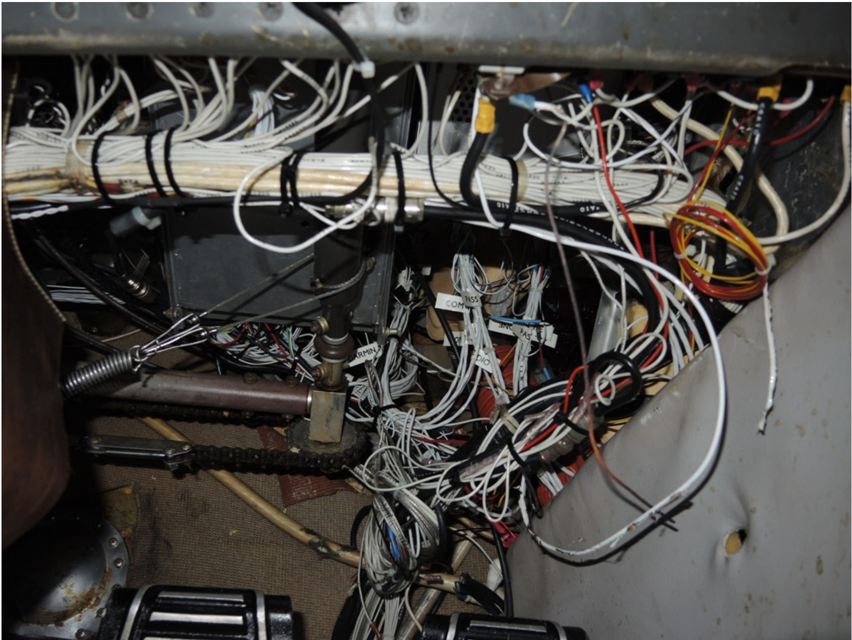
Photo 9 - Textron Aviation Photograph. View of the Co-Pilot Side Lower Instrument Panel.
