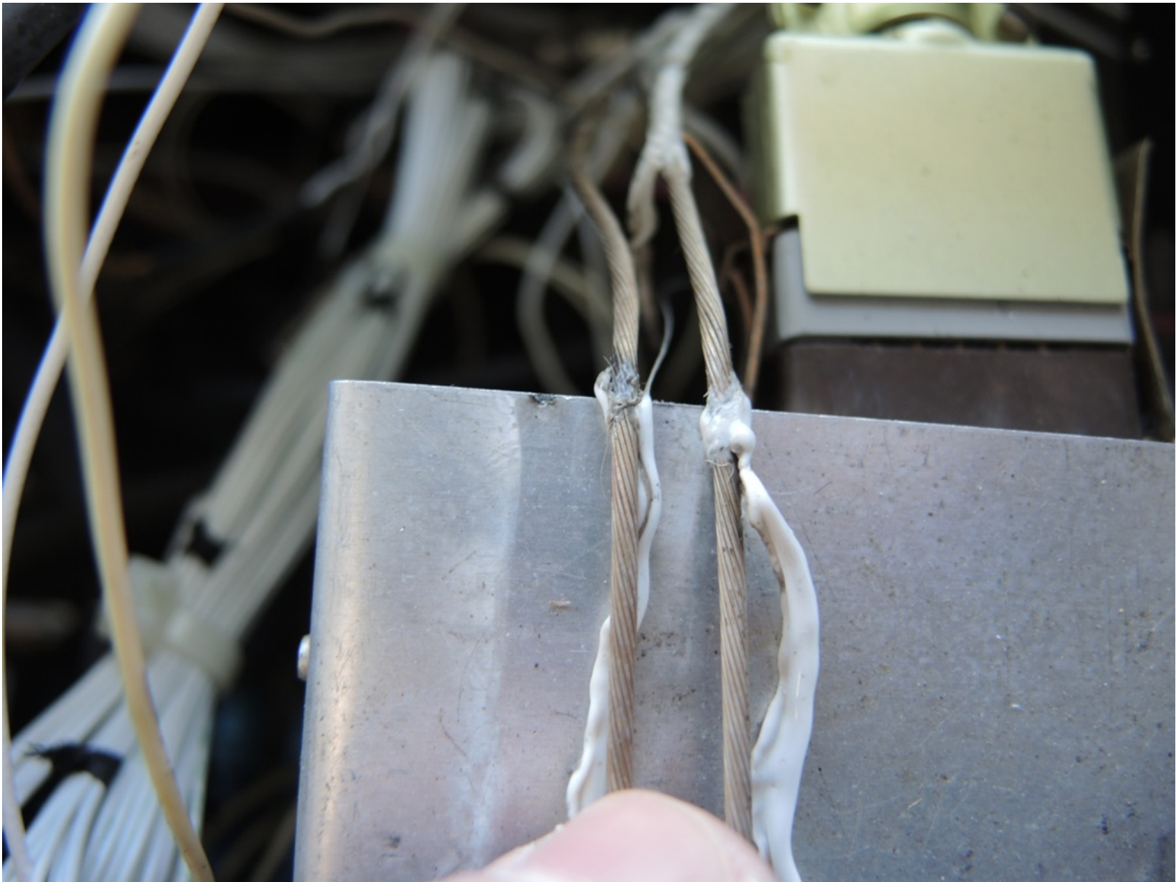
Photo 10 - Textron Aviation Photograph. View of the Arcing damage to the Electrical Wire of the Avionics Master Switch and the Aft Portion of the Adjacent Autopilot Control Unit.
