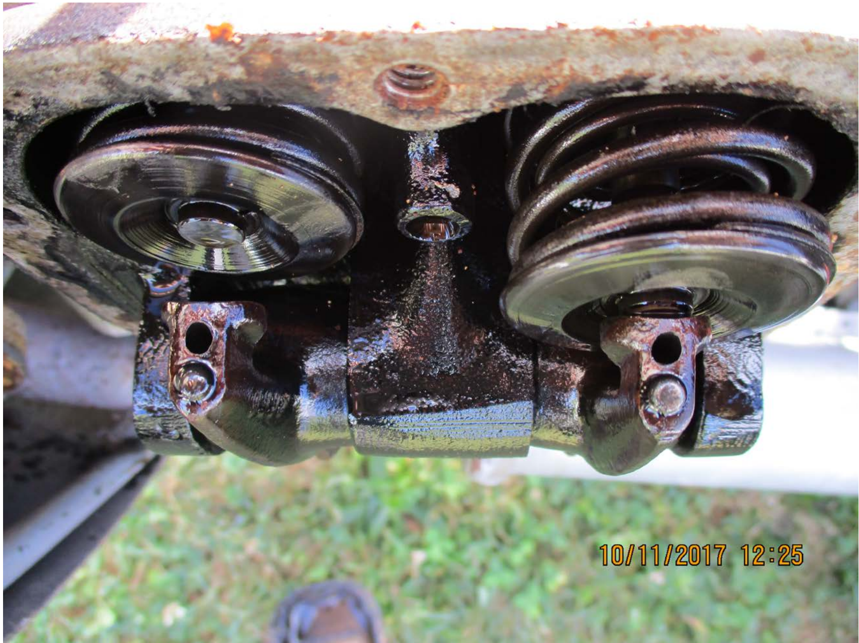
Photo 2 – View of #2 Exhaust Valve in Compressed (Open) Position (FAA)
