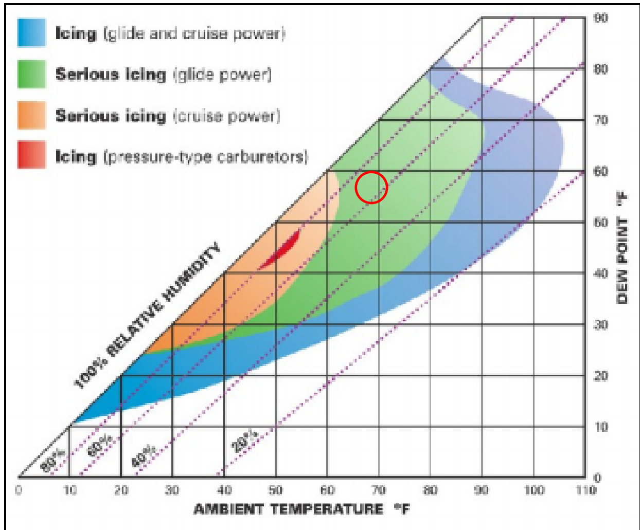
FAA Carburetor Icing Probability Chart
