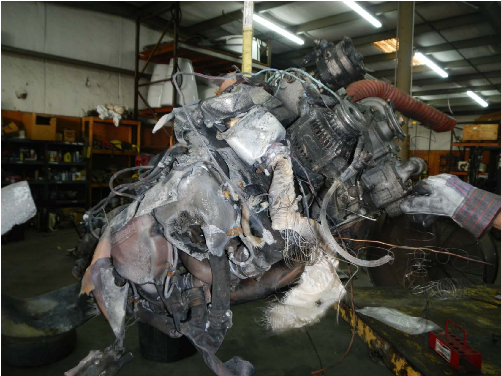
Photo 13 – View of left side engine showing impact and fire damage
