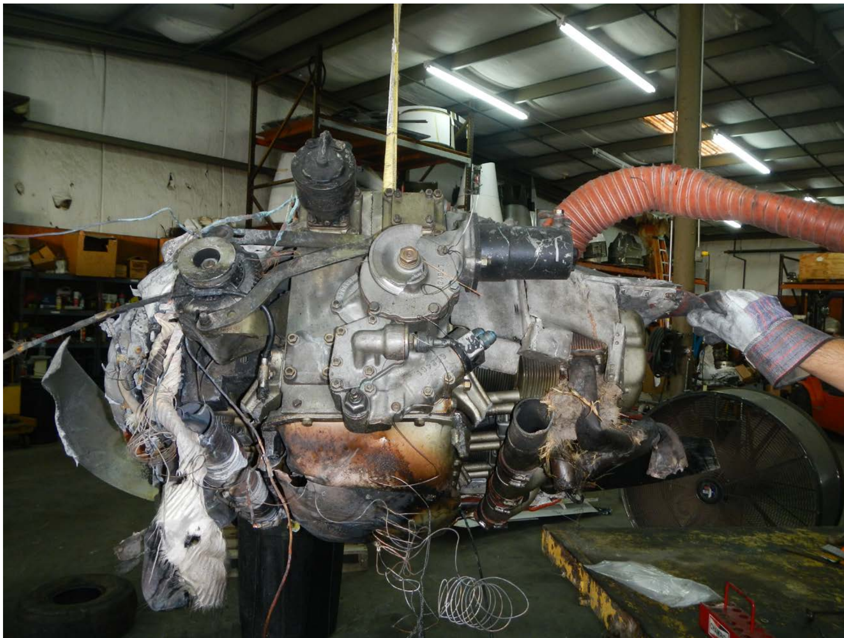
Photo 14 – View of accessory section showing impact and fire damage
