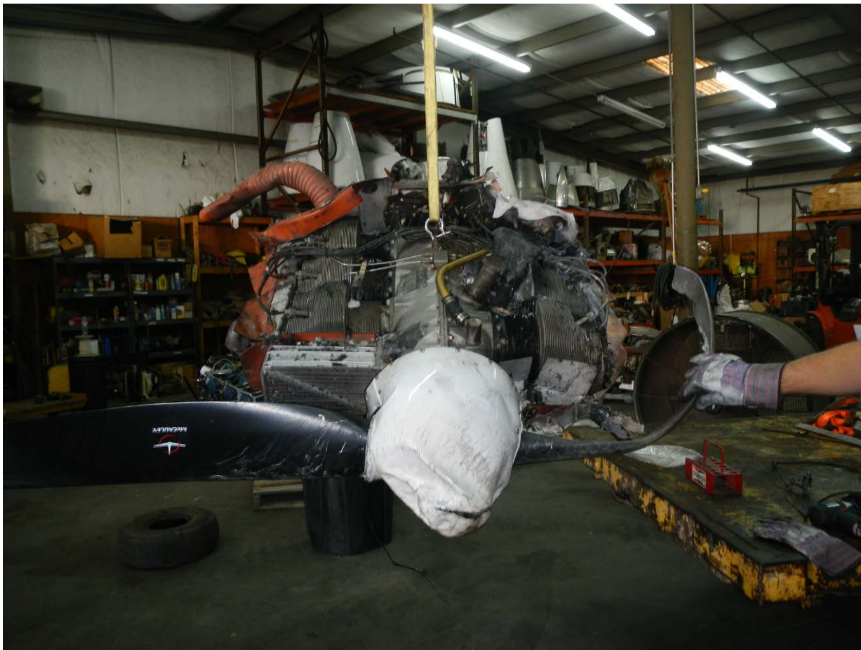
Photo 11 – View of front of engine and propeller showing impact damage
