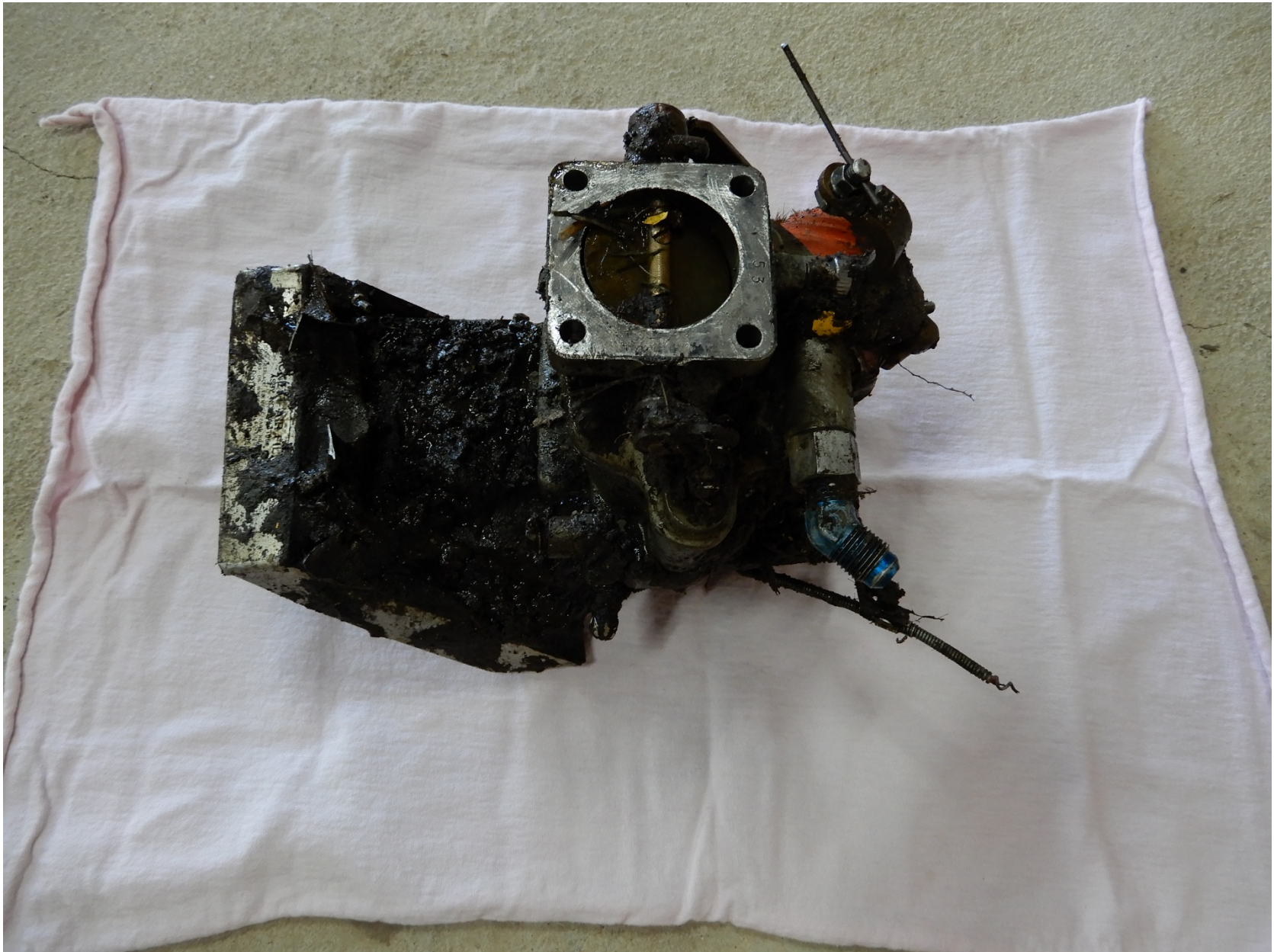
Photo 6 – View of Carburetor and Air Box
