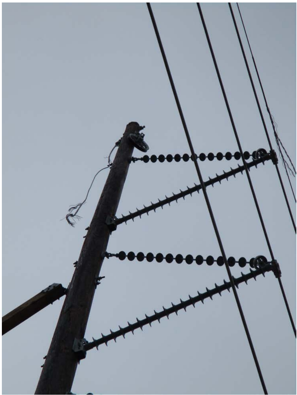
Photo 6 – View of Partially-Wrapped Armor Rod on Static Line as Found (FAA)
