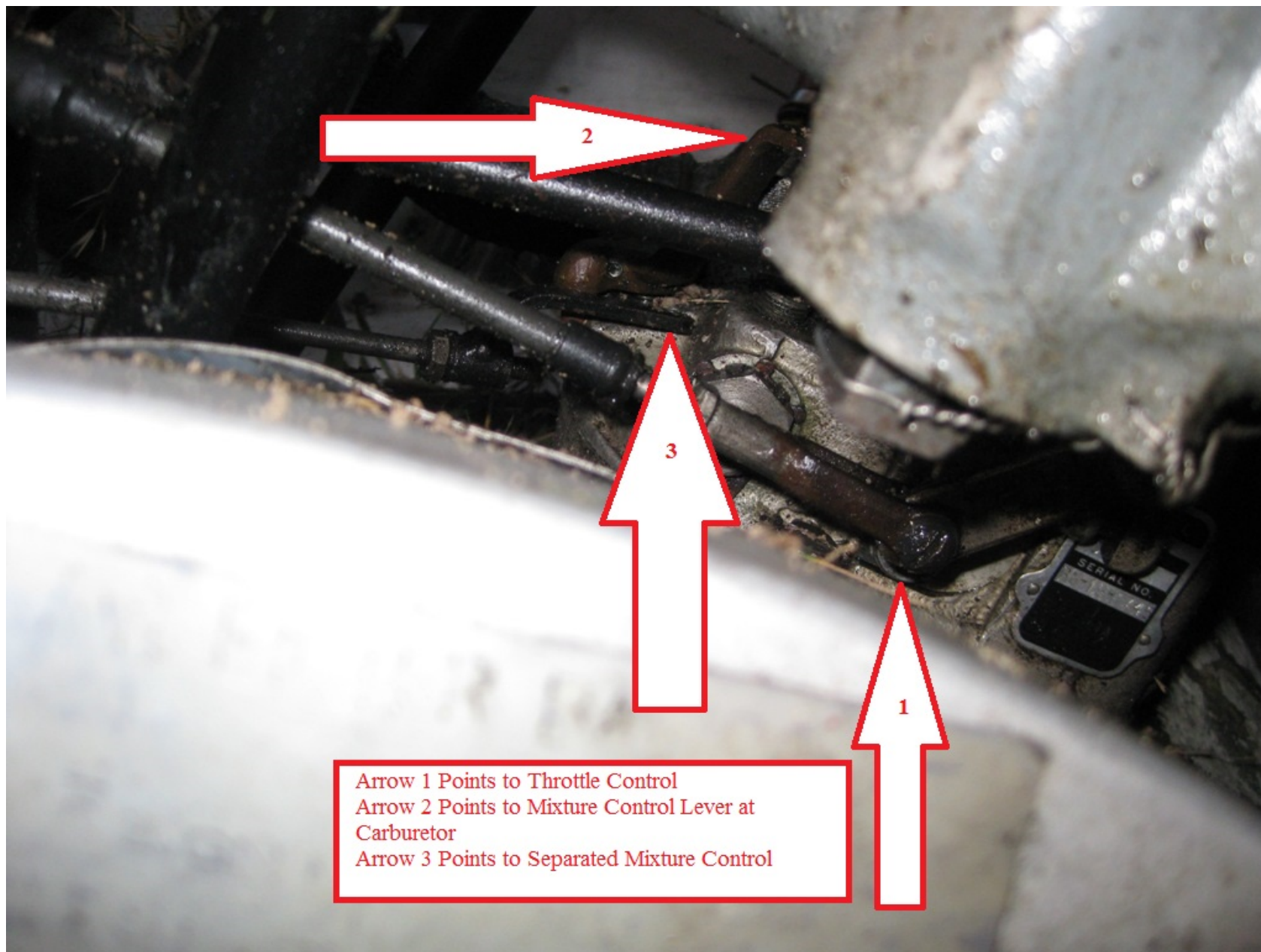
Photo 3 – FAA Digital Photograph with Captions Added by NTSB. View Depicting the Connected Throttle Control and Separated Mixture Control at the Carburetor
