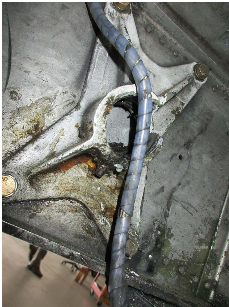
Photo 1 – View of fractured right main landing gear trunnion
