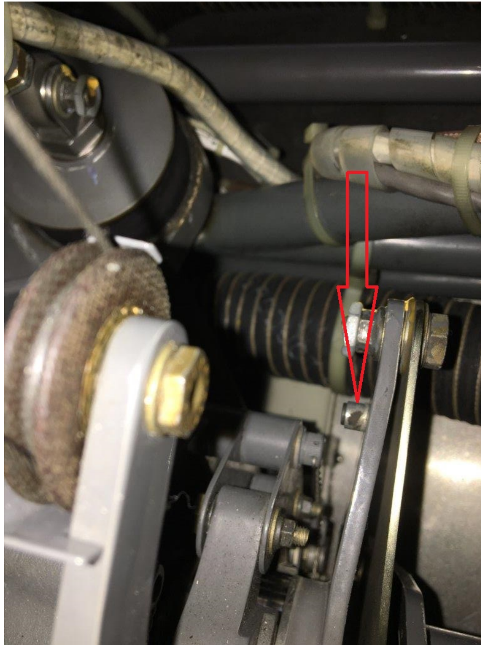
Photo 3 – Digital Photograph Provided by FAA. Red Arrow Points to 1 Magnet Assembly Installed in C908-1 Yoke Assembly.
