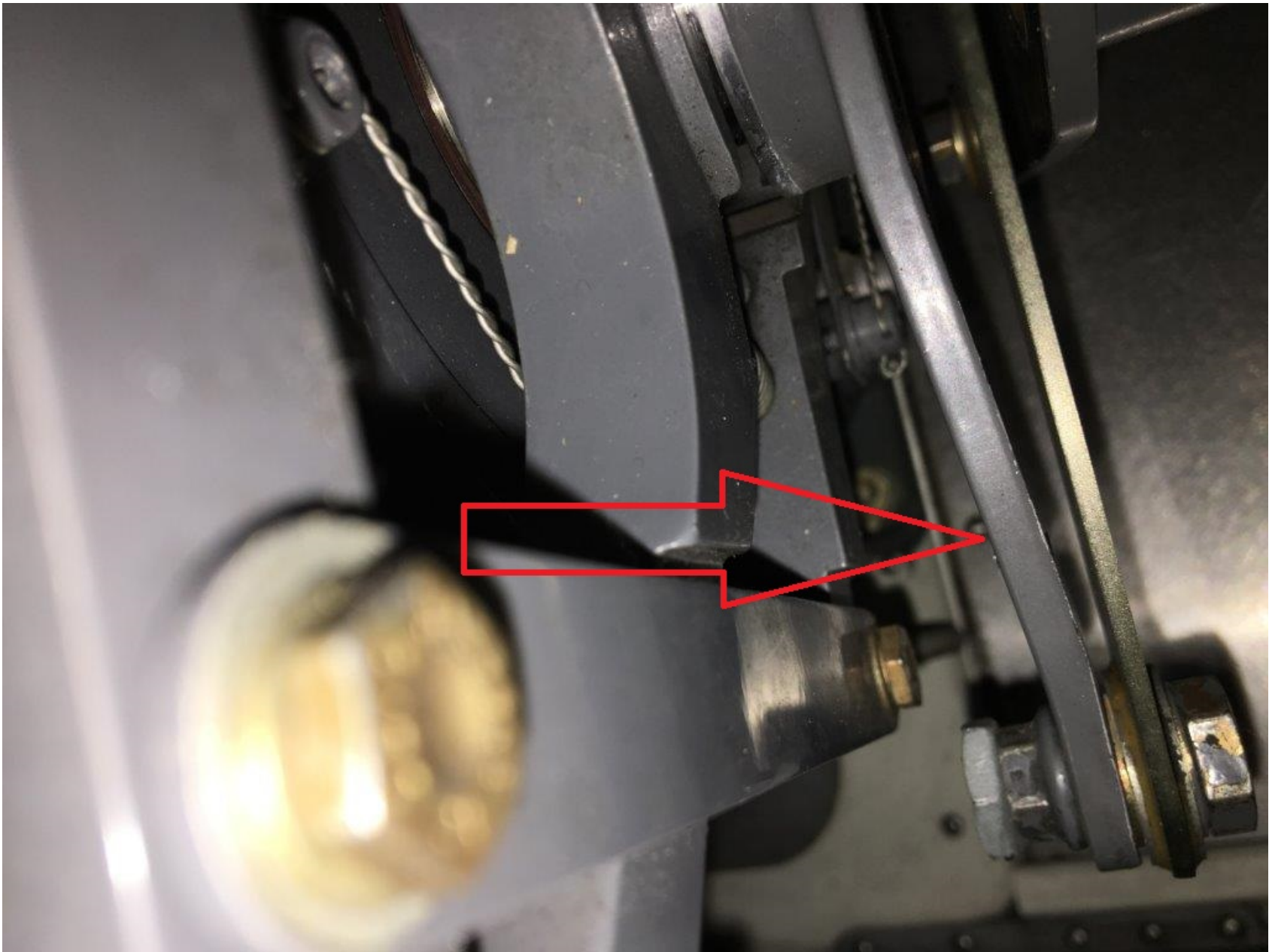
Photo 4 - Digital Photograph Provided by FAA. Red Arrow Points to Area on C908-1 Yoke Assembly with Missing Magnet Assembly.
