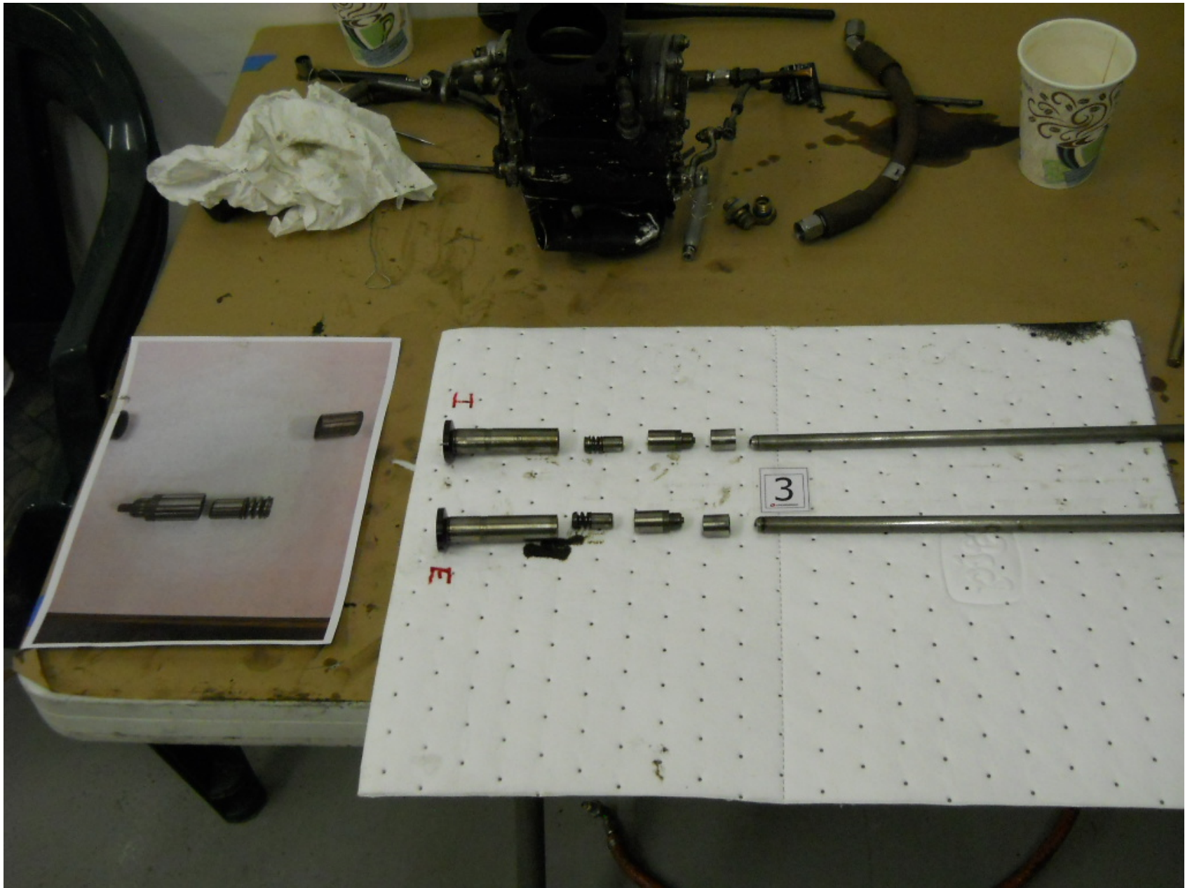
Photo 4 - #3 Cylinder Tappet Assembly (NTSB)
