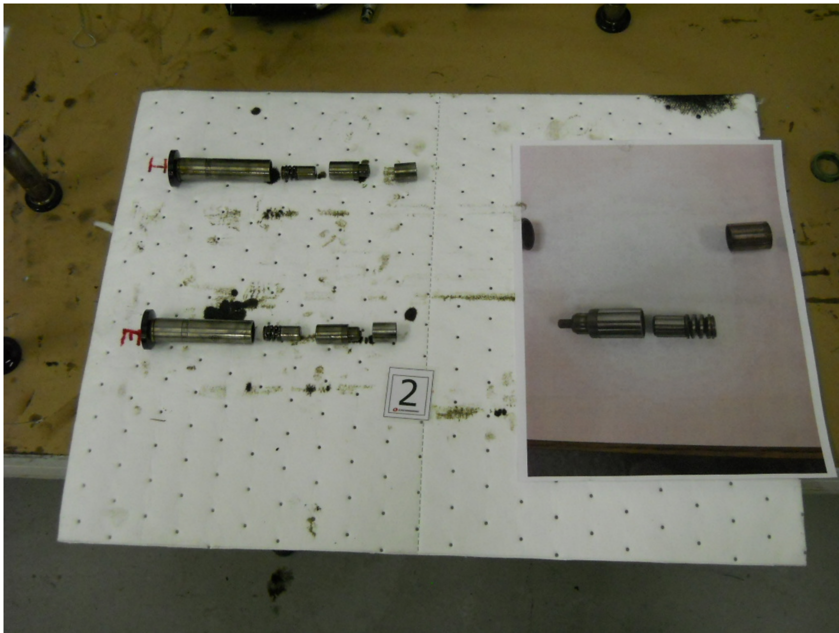
Photo 5 - #2 Cylinder Tappet Assembly (NTSB)
