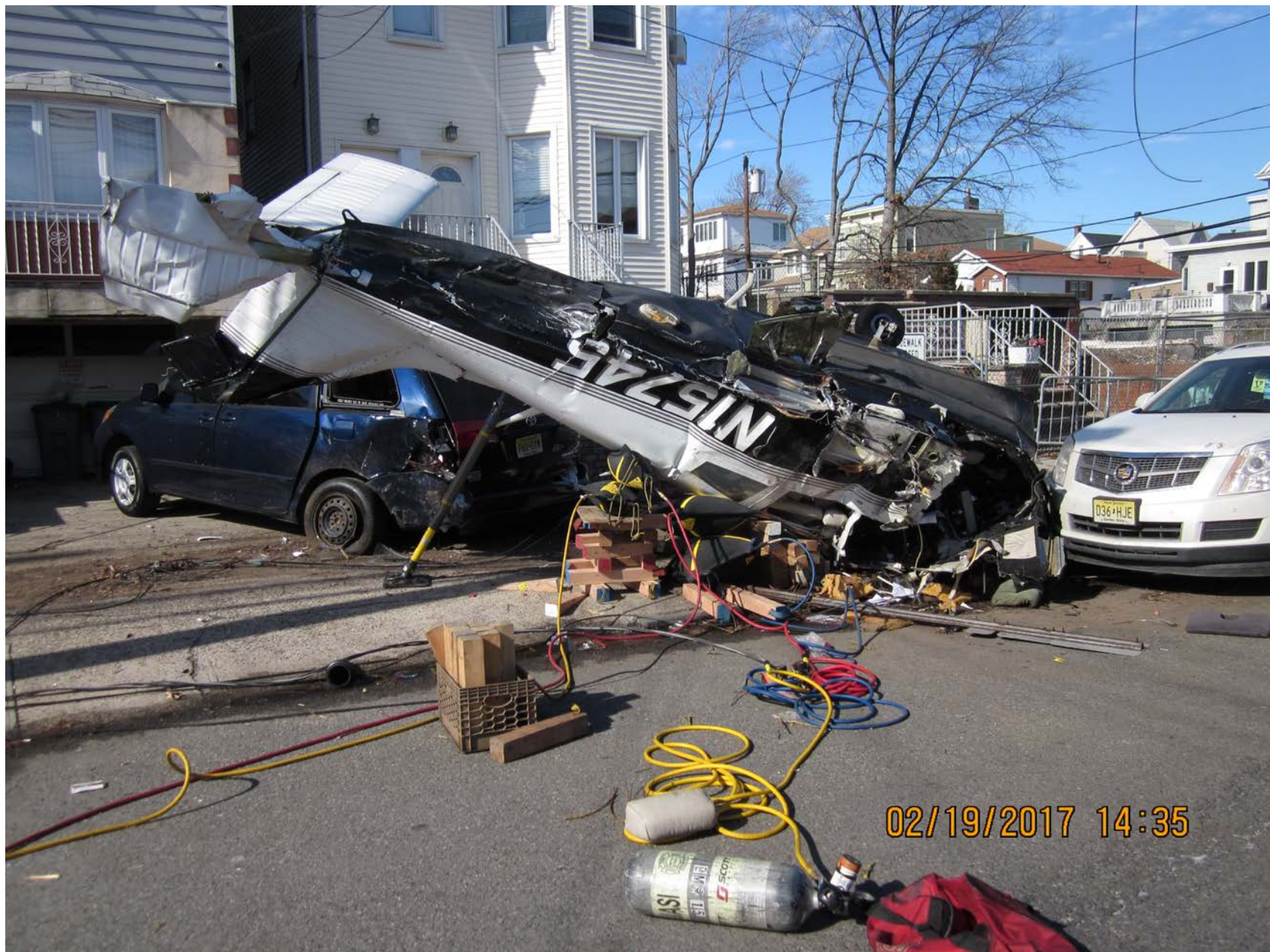
Photo 1 – Airplane Wreckage inverted at Accident Site (FAA)
