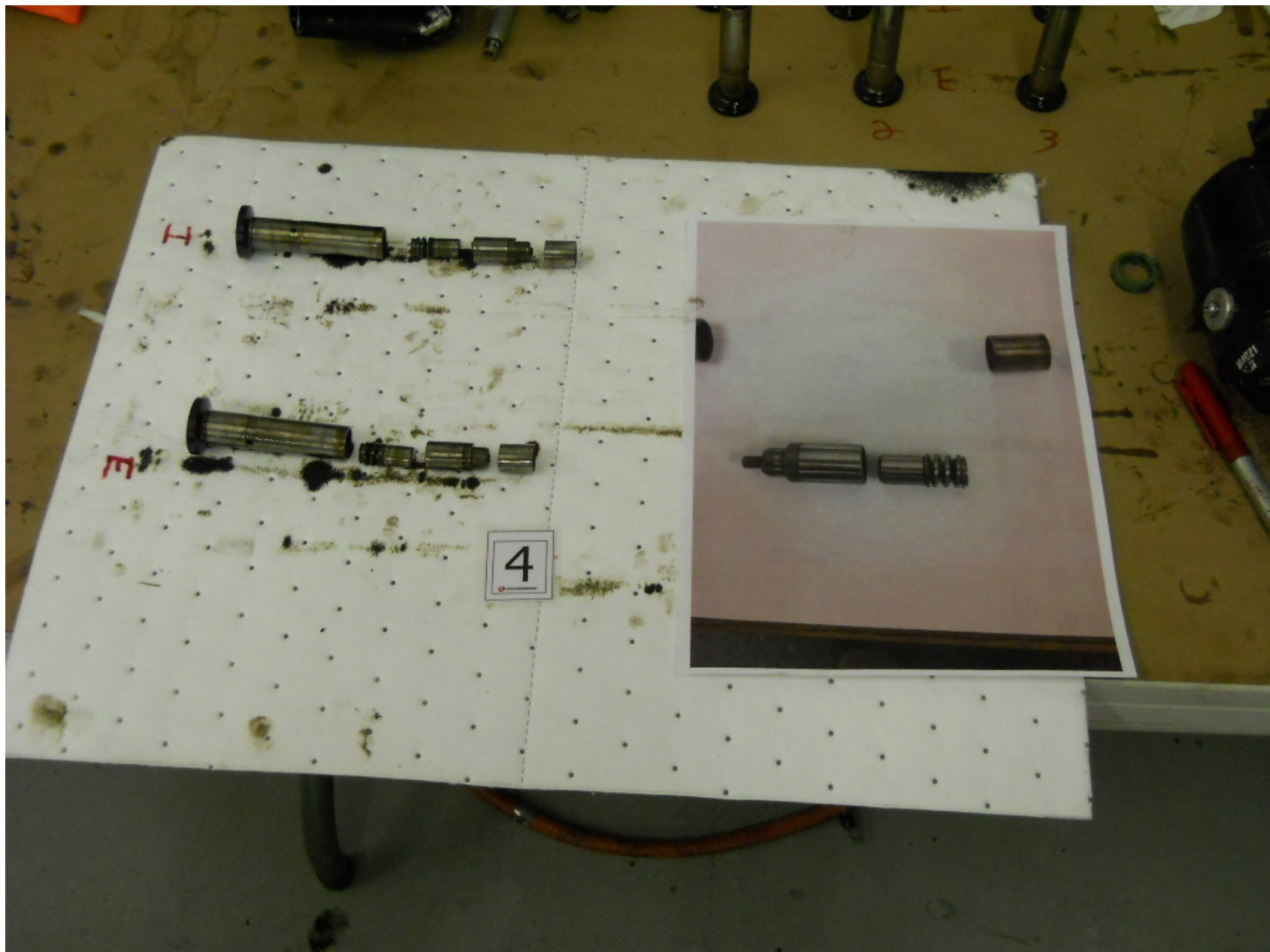
Photo 7 - #4 Cylinder Tappet Assembly (NTSB)
