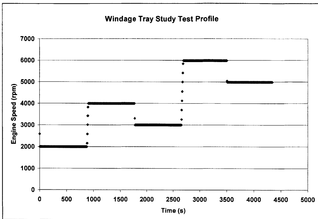
Figure 4-5 Windage tray study test profile
