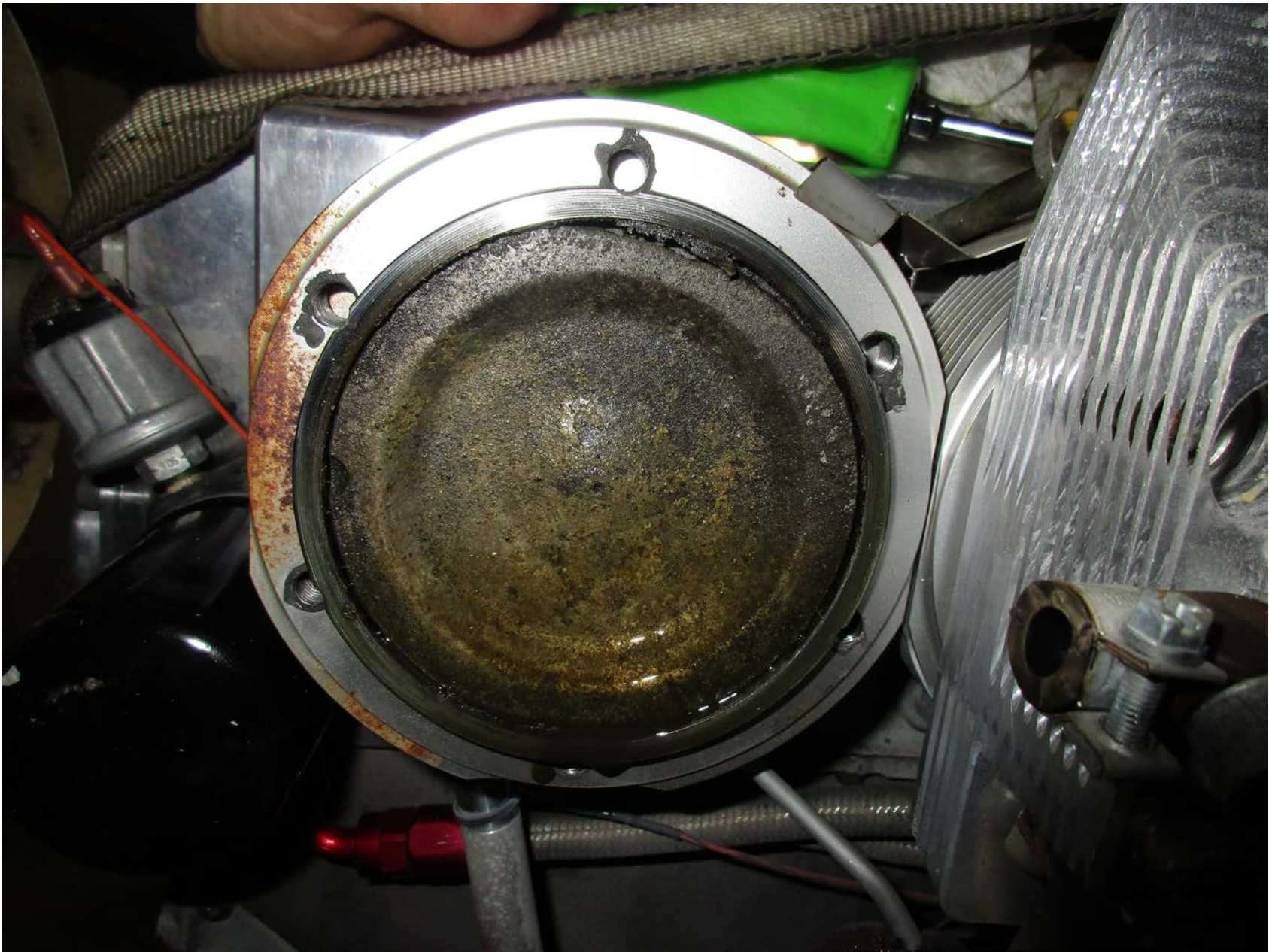
Photo 3 - Photo From FAA. View of the No. 2 Cylinder Piston and Barrel. Note the Erosion of the Piston Edge Near the 1 O'Clock Position.
