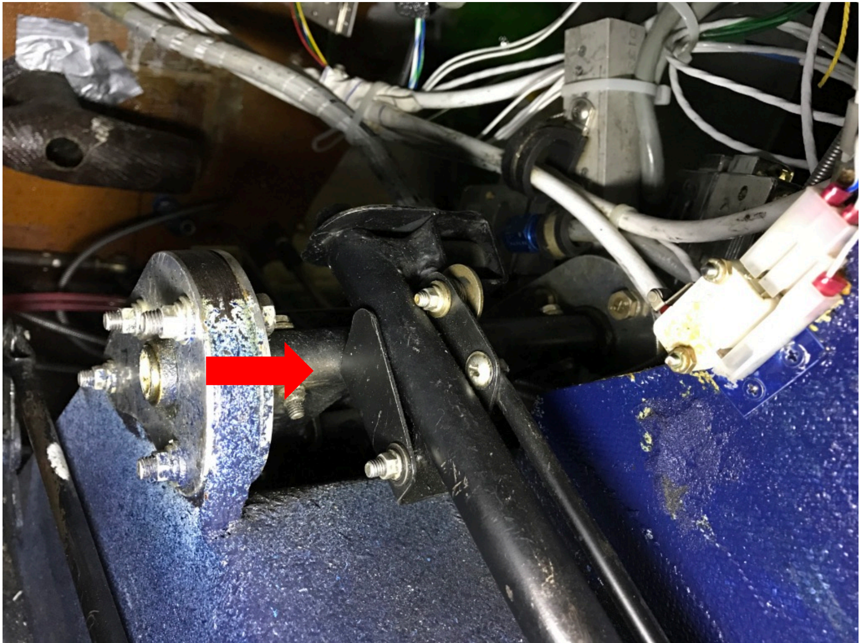
Photo 13 – Nose Gear Down Lock Displaying Minimal Contact with Pivot Shaft – Courtesy of FAA
