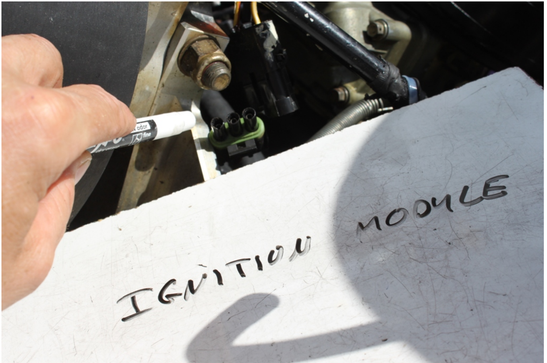
Photo 9 - NTSB Digital Photograph. View Depicting the Separated Electrical Connection at the Ignition Control Module.
