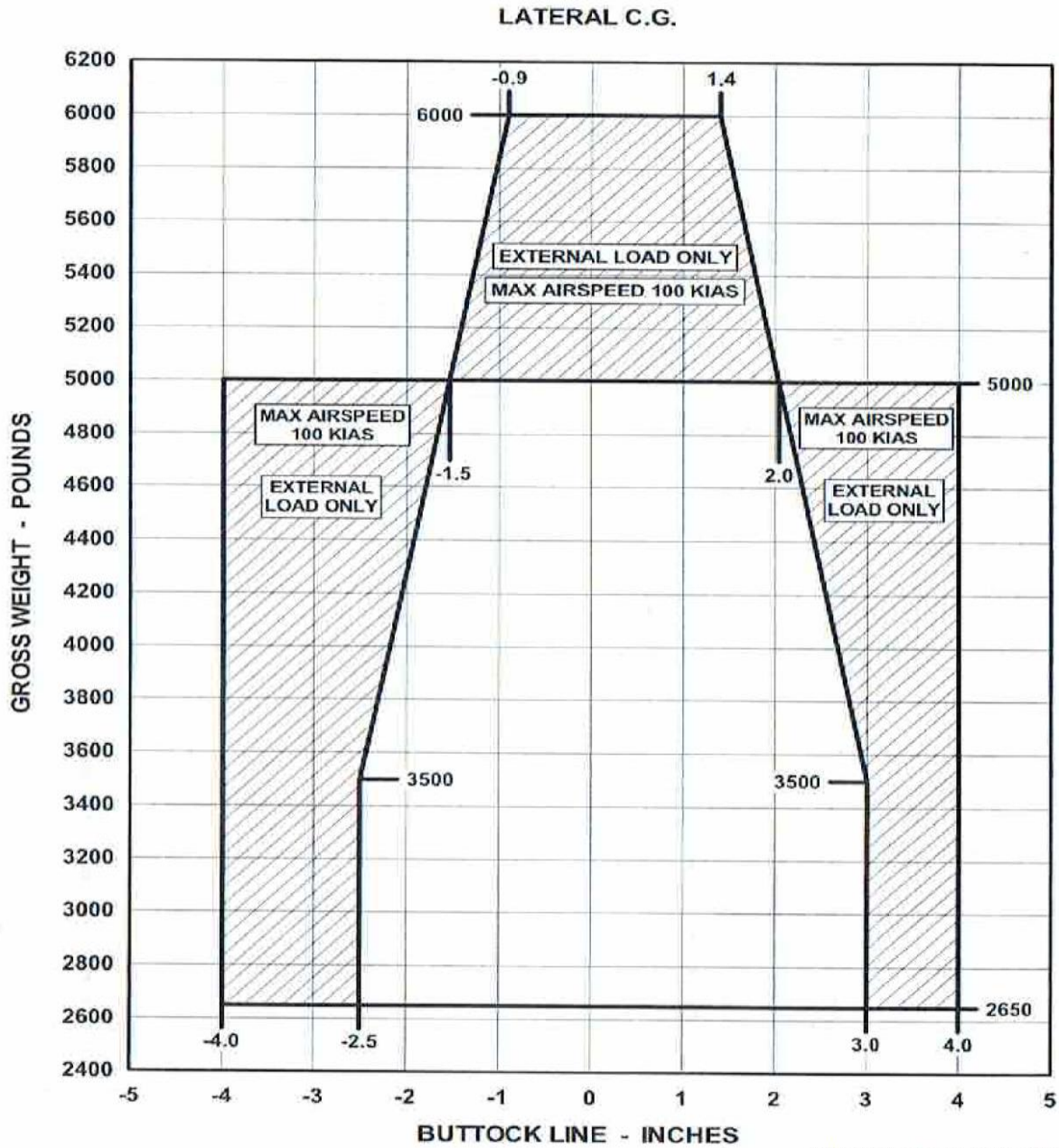
Figure 1-2. Gross weight lateral center of gravity limits (Sheet 1 of 2)
