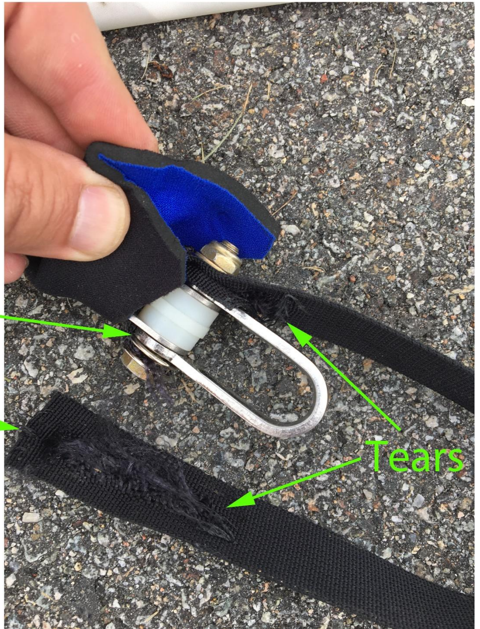
Cross Bar Restraint Cable – Shackle and Handle
