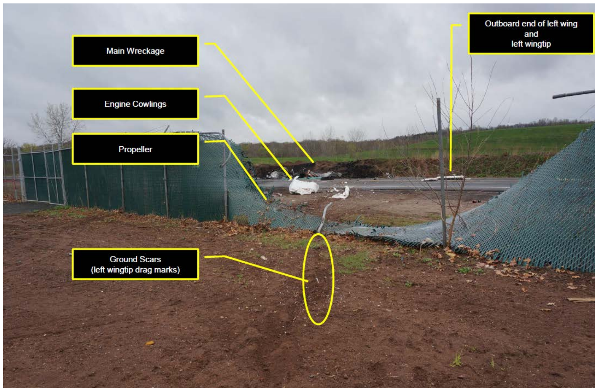
Photo 11 – Relationship of Ground Scars to the Debris Field – Courtesy of Cirrus Aircraft
