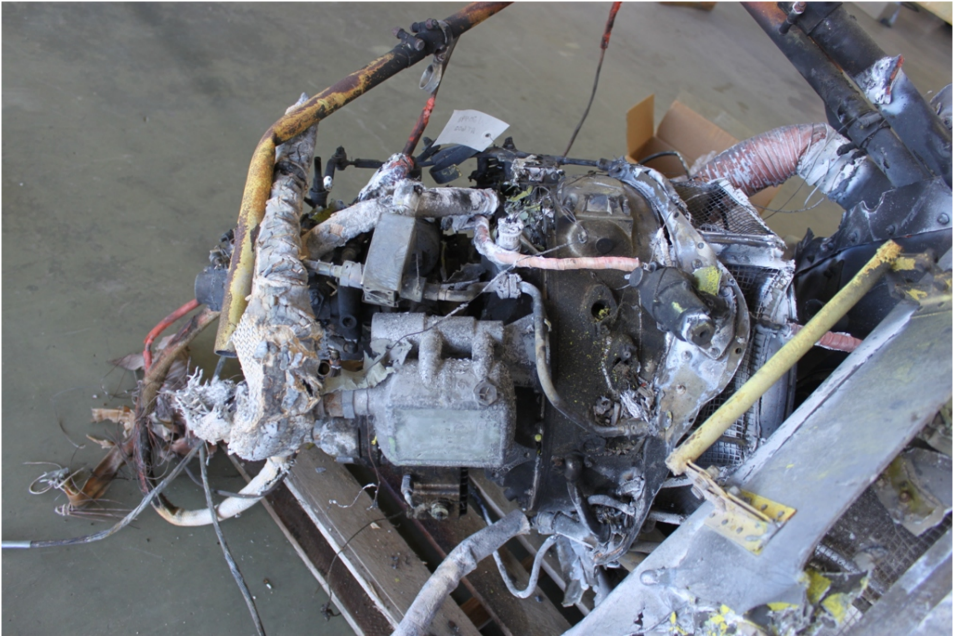
Photo 15 - NTSB Digital Photograph. Another View Depicting the Engine Assembly. Note the Heat Damage to the Hoses and Accessories
