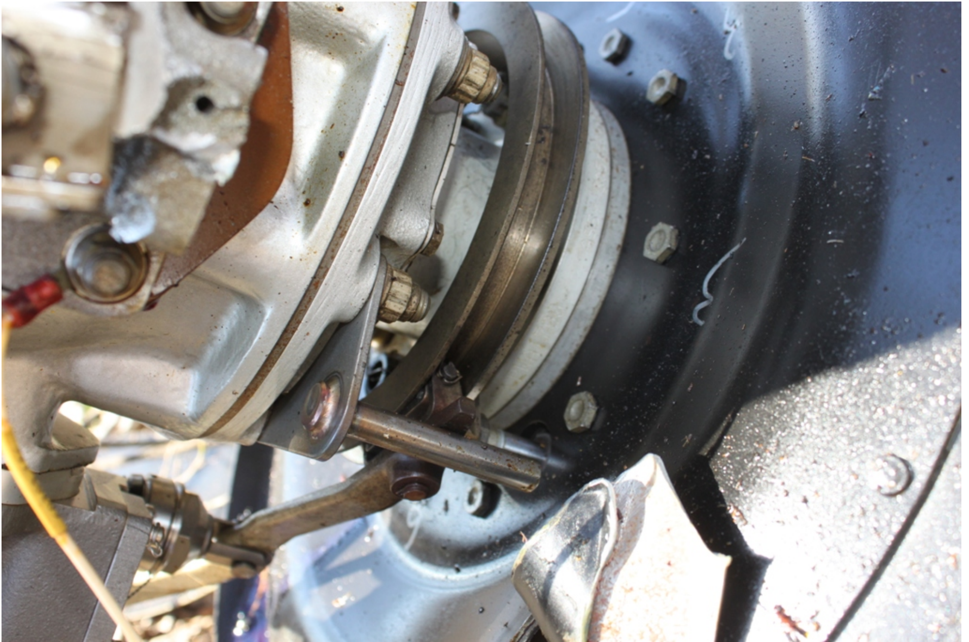
Photo 13 - NTSB Digital Photograph. View Depicting the Beta Block In Proper Relation to the Guide Pin
