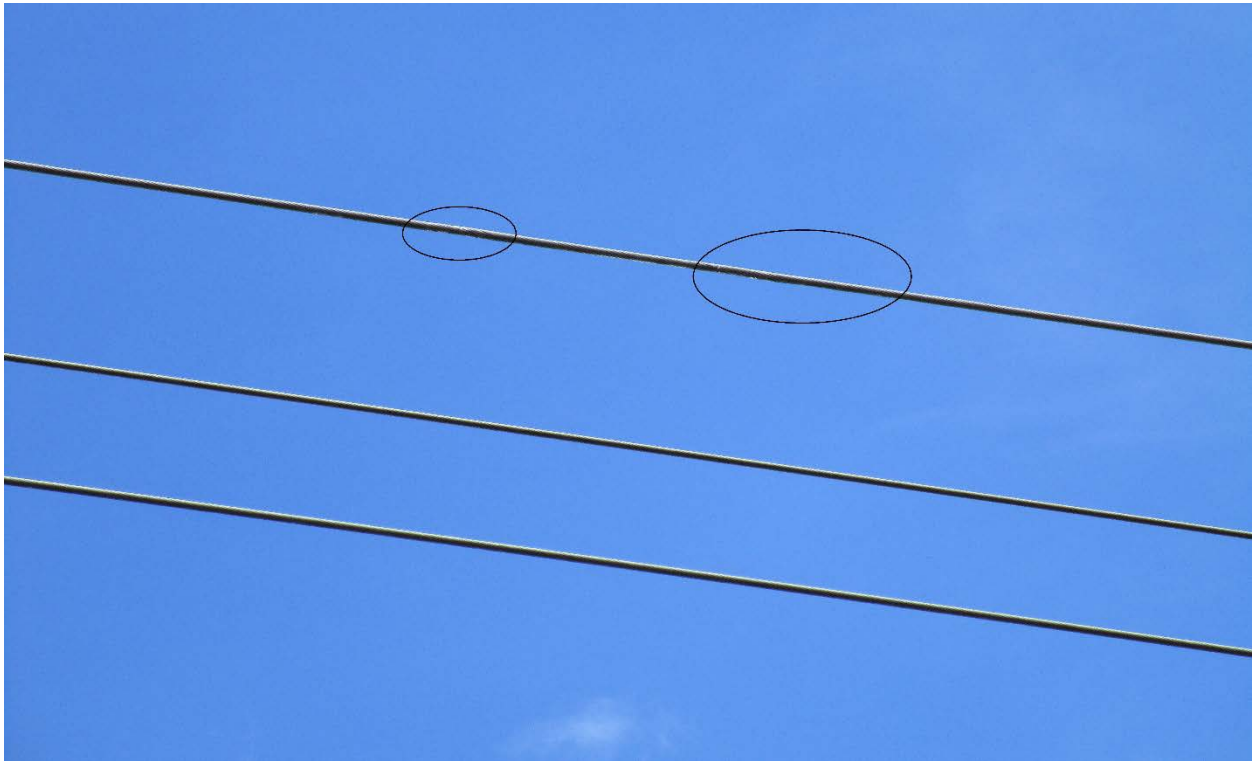
Figure 5 Striations on the power lines directly above the aircraft wreckage. (Photo courtesy of the FAA)
