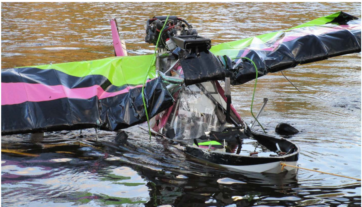
Figure 7 The airplane upright being pulled out of the river. (Photo courtesy of the FAA)
