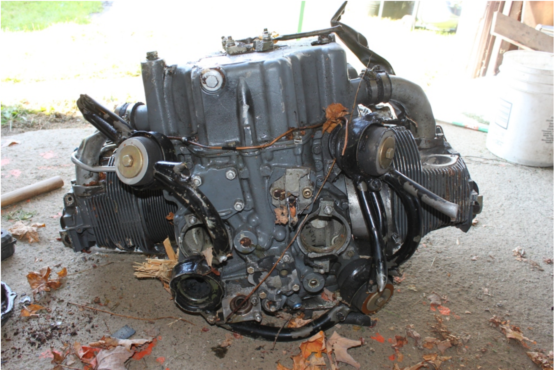
Photo 9 - NTSB Digital Photograph. View of the Rear Portion of the Inverted Engine Following Recovery. Note the Missing Engine Accessories.
