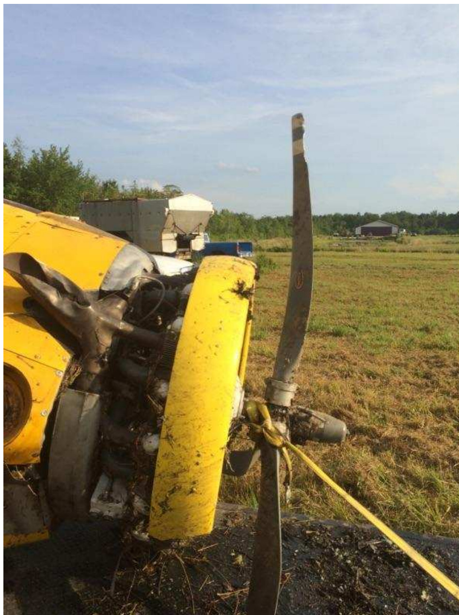
Photo 1 – Side view of engine with bird feathers in cowling. (Courtesy of FAA)
