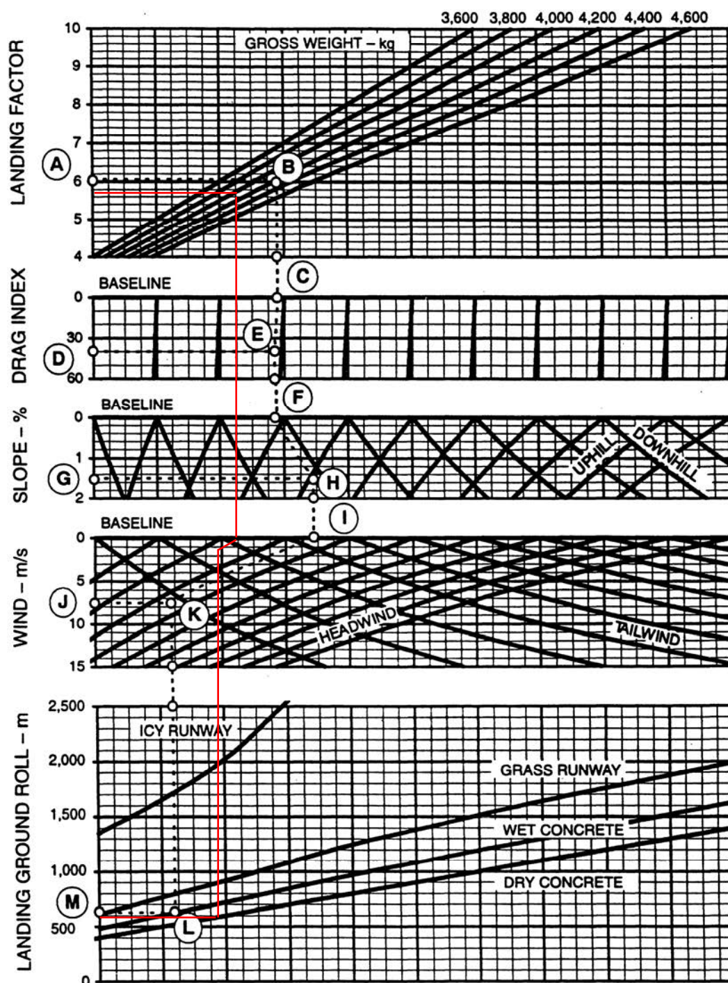
Figure A7-3. Landing Ground Roll
