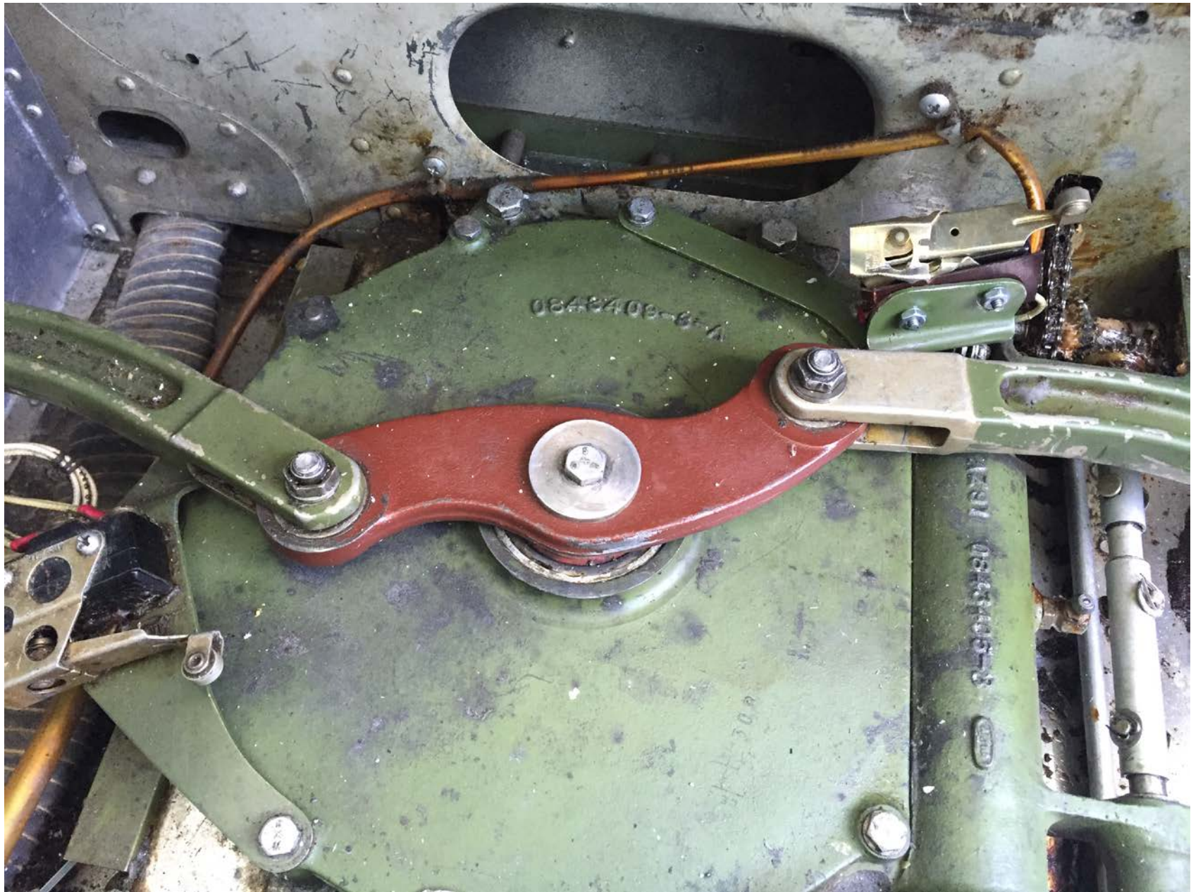
Photo 6 – Close-up View of Actuator as Found (FAA)
