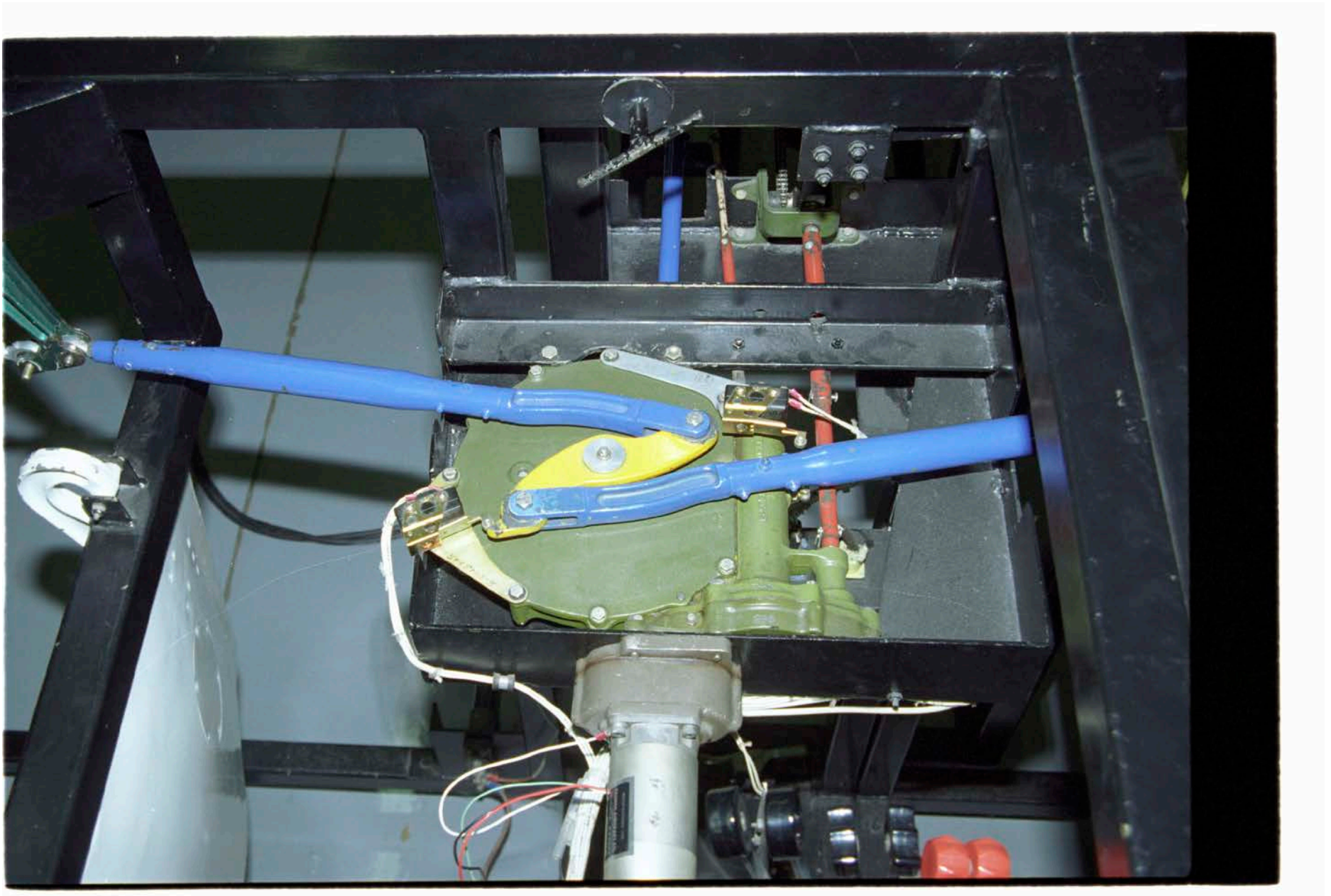
Photo 3 – View of Exemplar Landing Gear Actuator Retracted Position (Textron)
