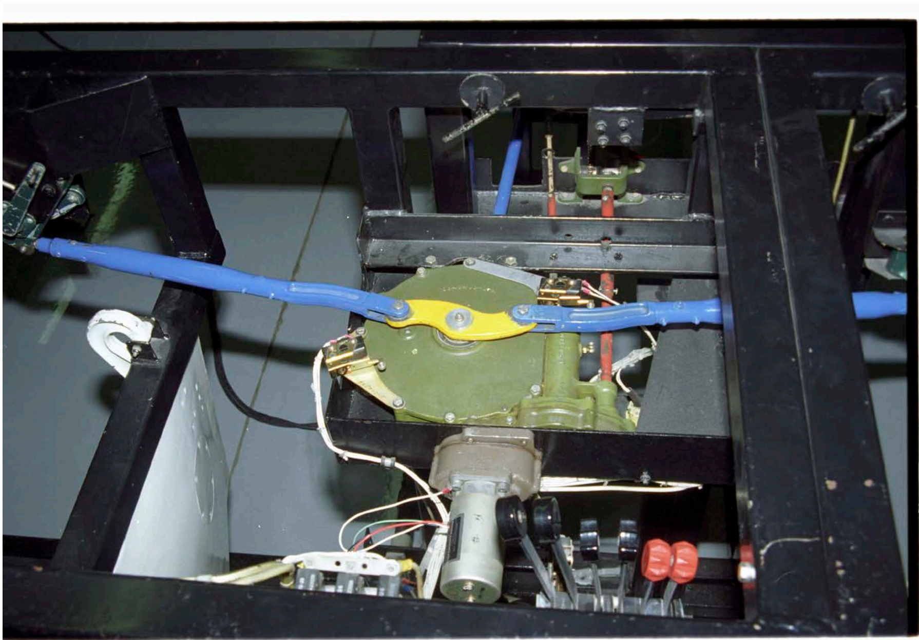
Photo 4 - View of Exemplar Landing Gear Actuator Extended Position (Textron)
