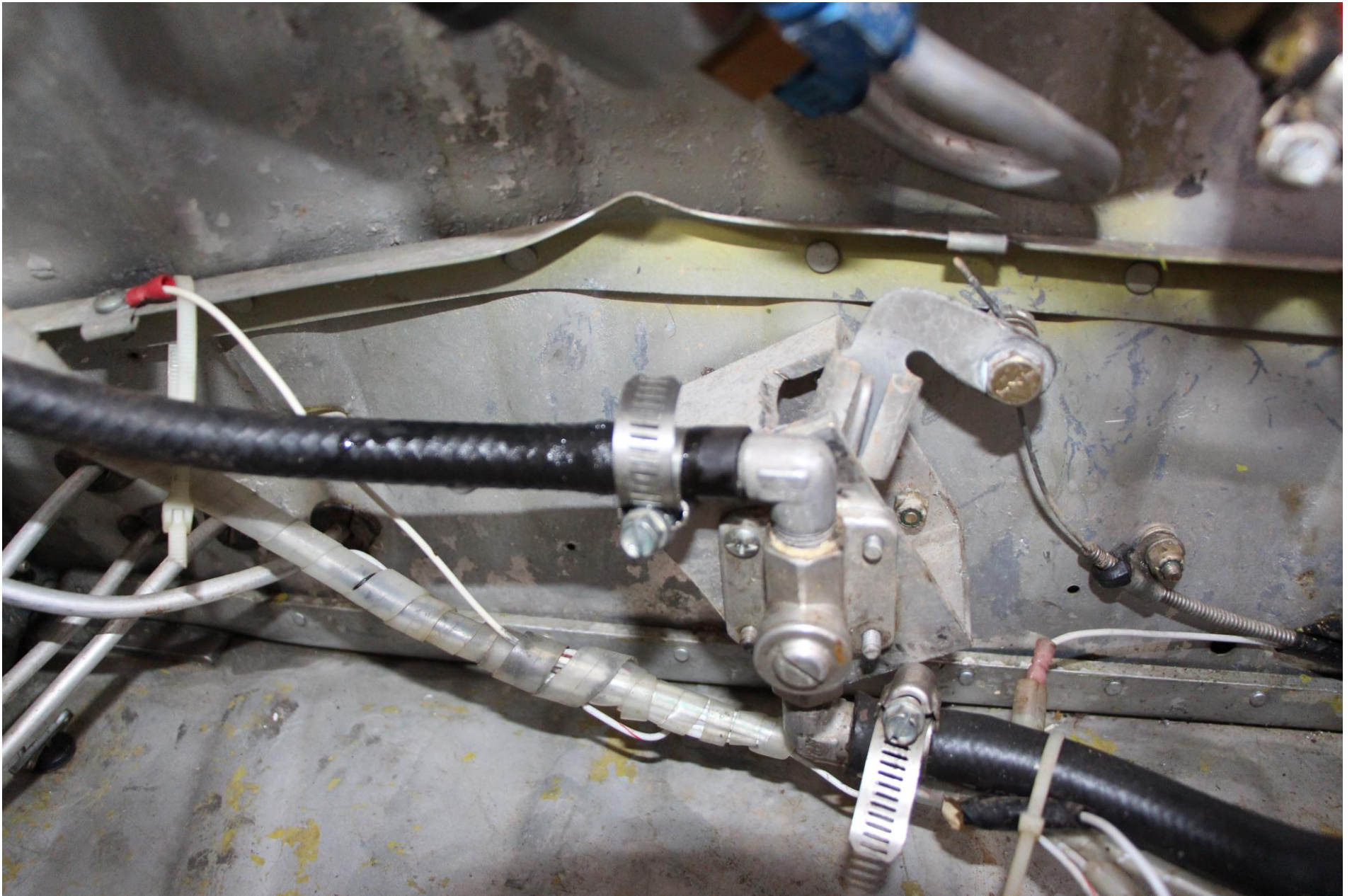
Photo 3 – loose fuel line with fuel leaking
