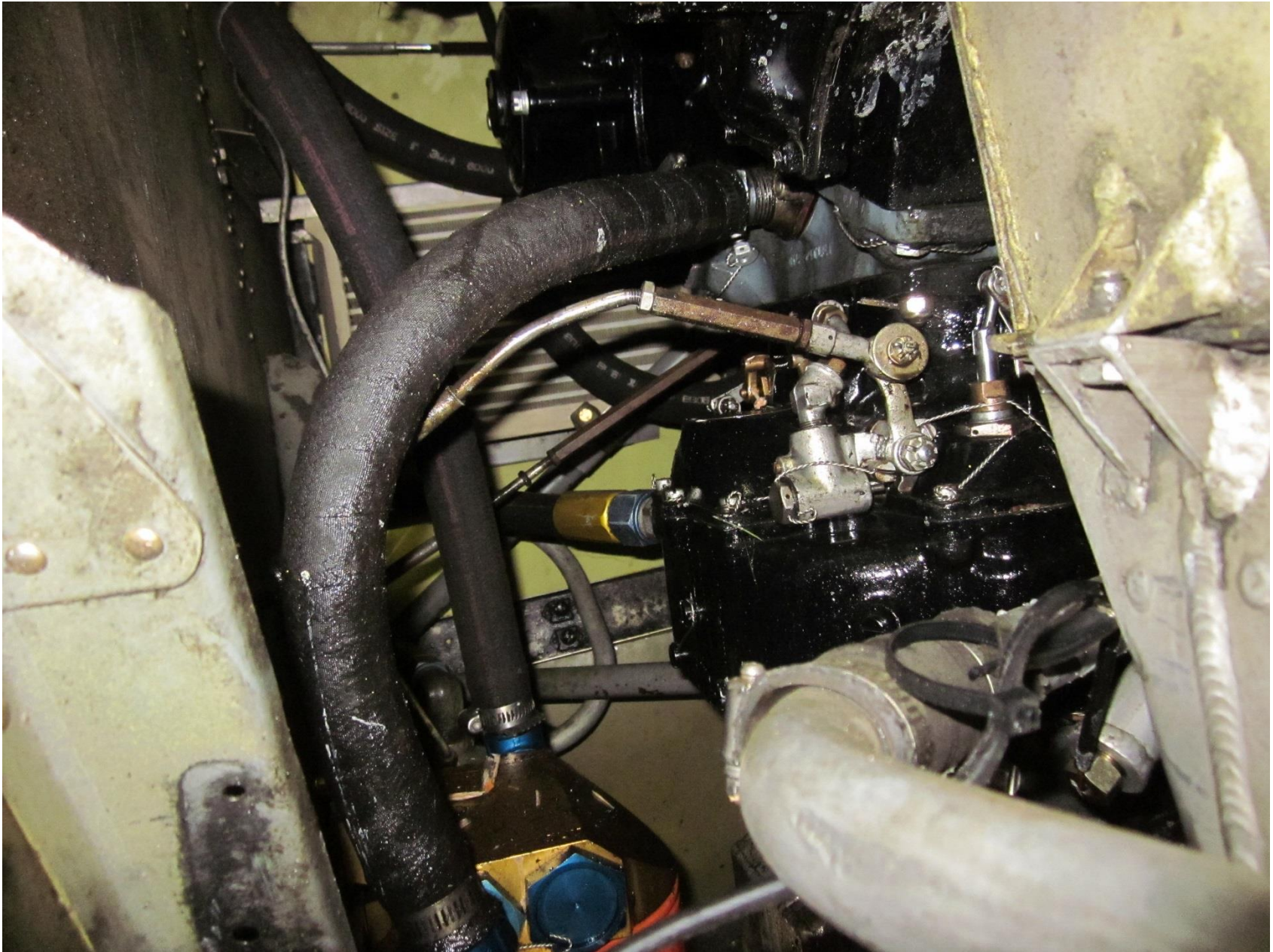
Photo 6 – Throttle Linkage (FAA Photo)
