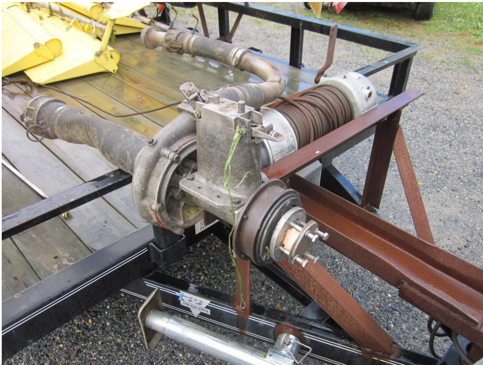
Photo 5 – Spray Pump (FAA Photo)
