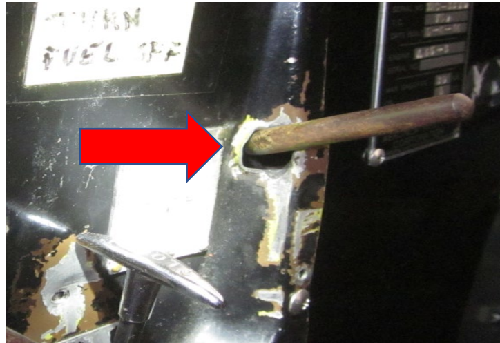
Accident Airplane Fuel Shutoff (Note: Missing Grommet)
