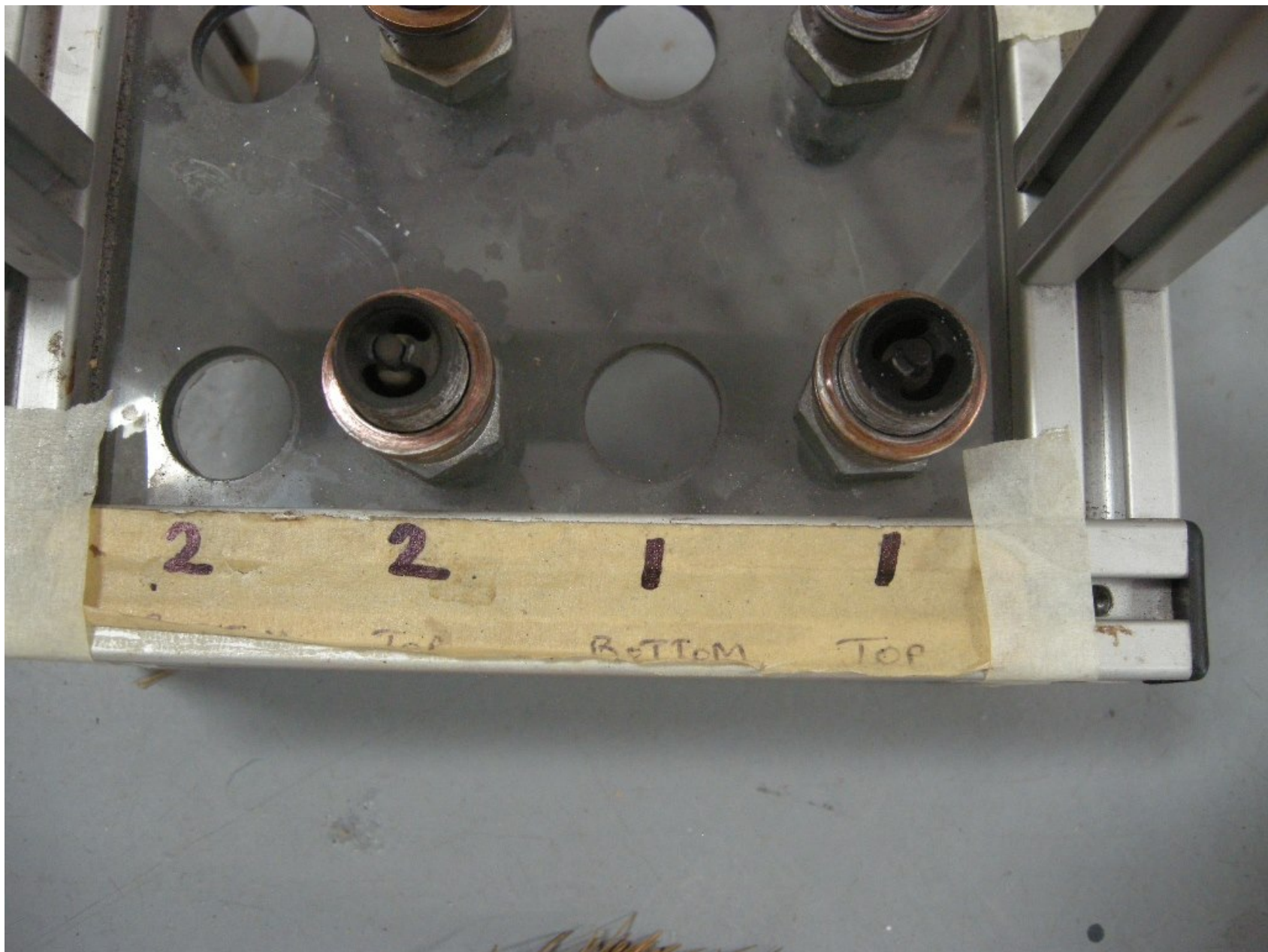
Photo 4 – Numbers 1 and 2 Top Spark Plugs (NTSB Photo)
