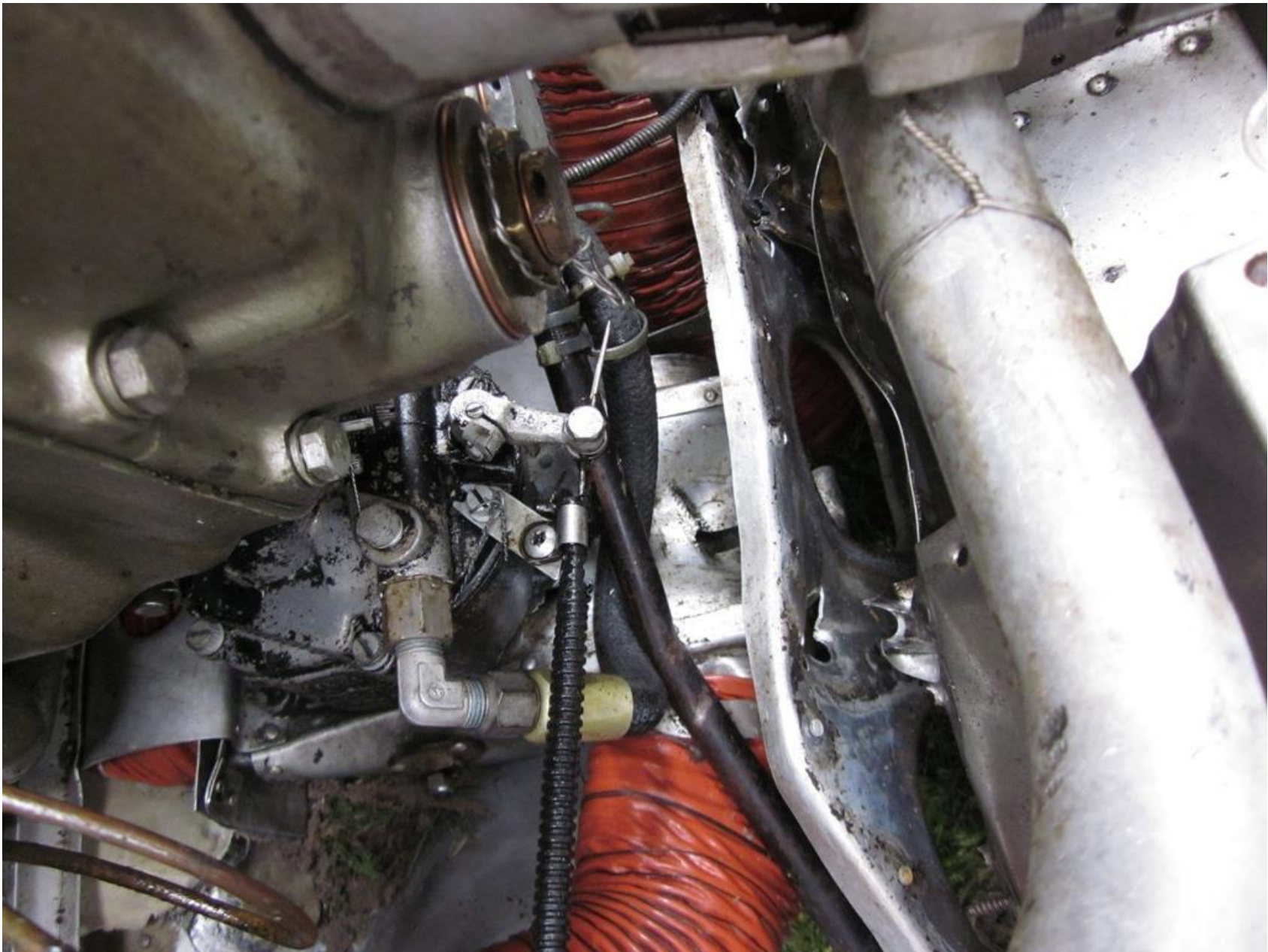
Photo 4 - FAA Digital Photograph. View Depicting the Position of the Mixture Control at the Carburetor Following Pulling of the Mixture Control Full Aft and then Pushing of the Mixture Control to Full Rich.
