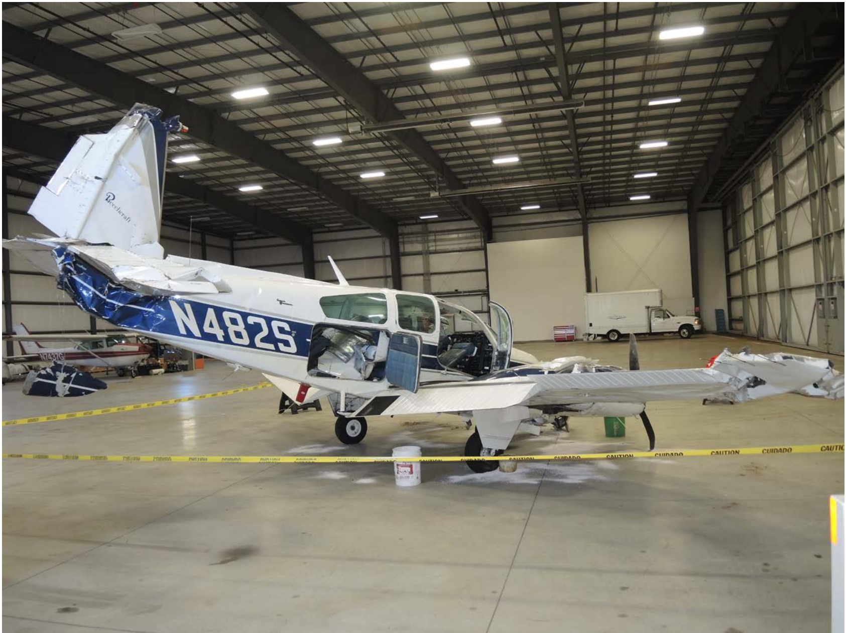
Photo 4 – Right Rear View of Airplane Damage (Courtesy of Textron)
