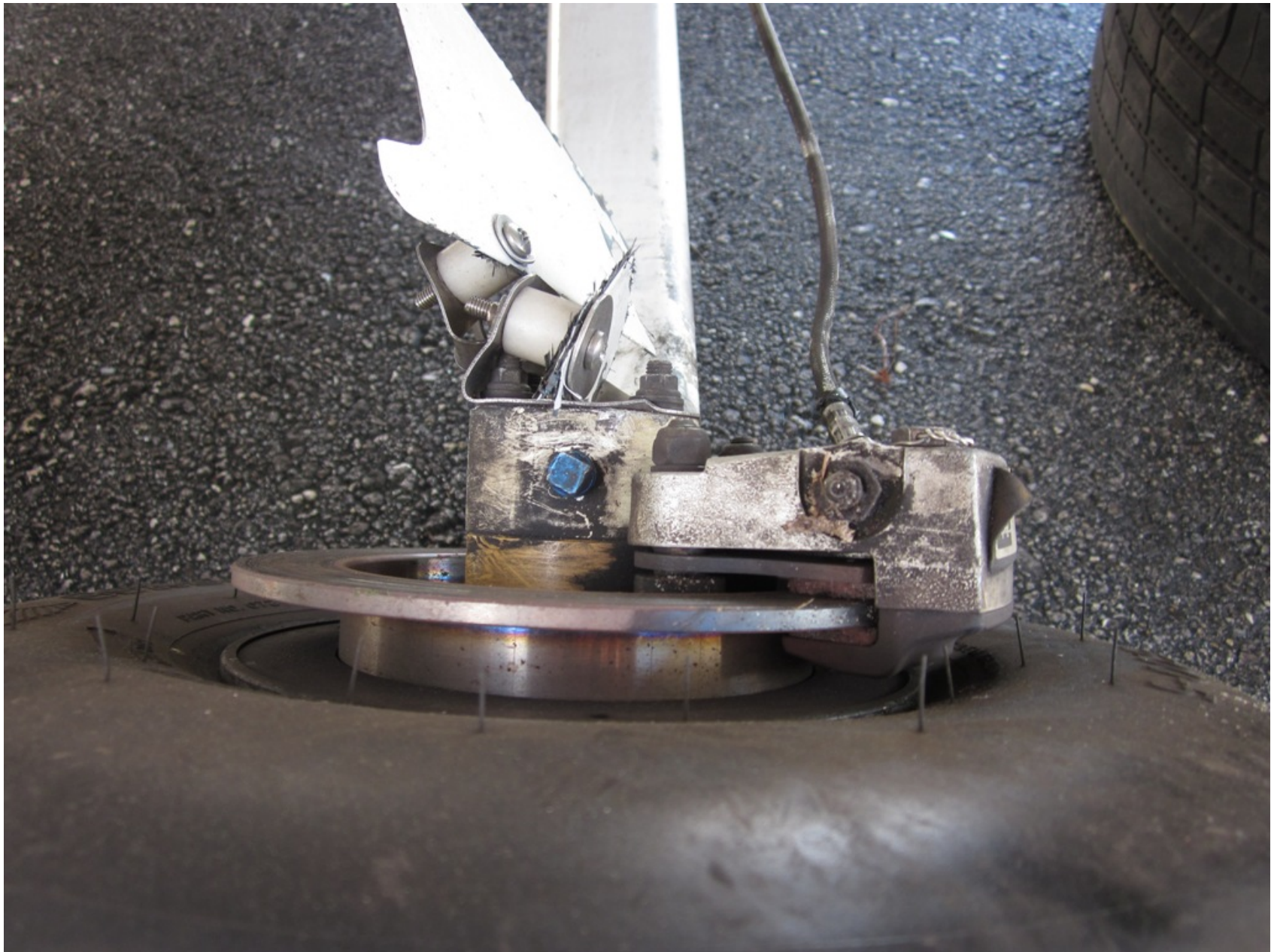
Photo 4 - FAA Digital Photograph. View Depicting the Right Brake Caliper, Brake Disk, and Portion of Right Tire. Note the Blue Discoloration on portions of the Brake Disk
